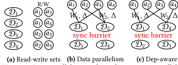
Figure 1. Data parallelism vs. dependence-aware parallelism: (a) the read-write (R/W) sets of data mini-batches \mathcal{D}_1 to \mathcal{D}_4 ; (b) in data parallelism, mini-batches are randomly assigned to workers, leading to conflicting parameter accesses; (c) in dependence-aware parallelization (note that \mathcal{D}_4 instead of \mathcal{D}_2 is scheduled to run in parallel with \mathcal{D}_1 ), mini-batches are carefully scheduled to avoid conflicting parameter accesses.
