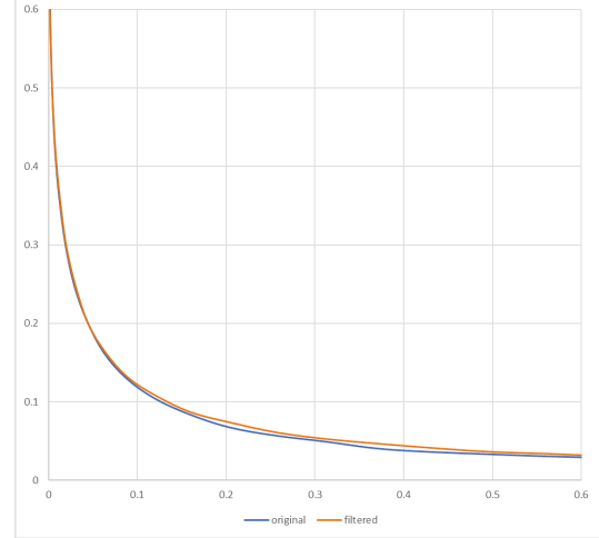
Figure 1. Detection Error Tradeoff (DET) for datasets with/without privacy filtering. X axis: FAR (false accepts) and Y axis: FRR (false rejects). Filtering privacy information slightly raises FRR.
