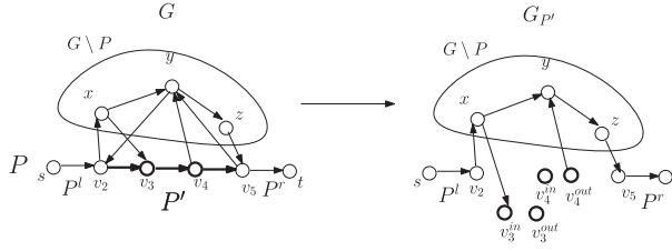
Fig. 2. An example of the transformation of a graph G into G_{P'} , given P and v_2 - v_5 subpath P' . Notice that edges (y, v_2) and (v_5, y) are removed, and that all nodes in W(P') = V(P') - \{v_2, v_5\} get split into two. The relevant paths in G_{P'} corresponding to detour paths circumventing edges in P are s \rightarrow v_2 \rightarrow x \rightarrow v_3^{in} , s \rightarrow v_2 \rightarrow x \rightarrow y \rightarrow z \rightarrow v_5 \rightarrow t , and v_4^{out} \rightarrow y \rightarrow z \rightarrow v_5 \rightarrow t .
