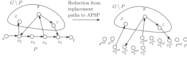
Fig. 1. An example of the reduction from RP to APSP in the case of an unweighted graph.
