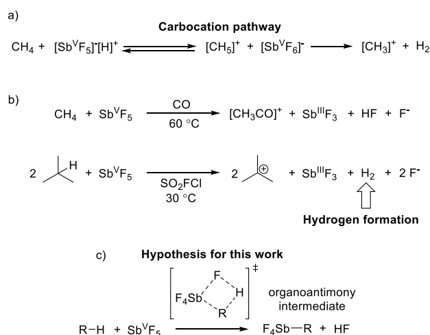
Scheme 1. a) Outline of methyl cation pathway for reaction of methane with [Sb V F 6 ][H] + . b) Overview of methane and isobutane oxidation reactions with SbF 5 . c) Possible C-H activation transition state and organoantimony intermediate as the first mechanistic step for the oxidation of alkanes by SbF 5 .
