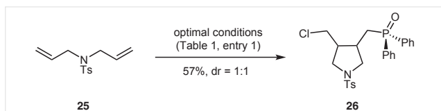
Scheme 3 Radical cyclization experiment
