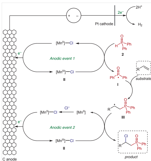
Scheme 4 Proposed mechanism
