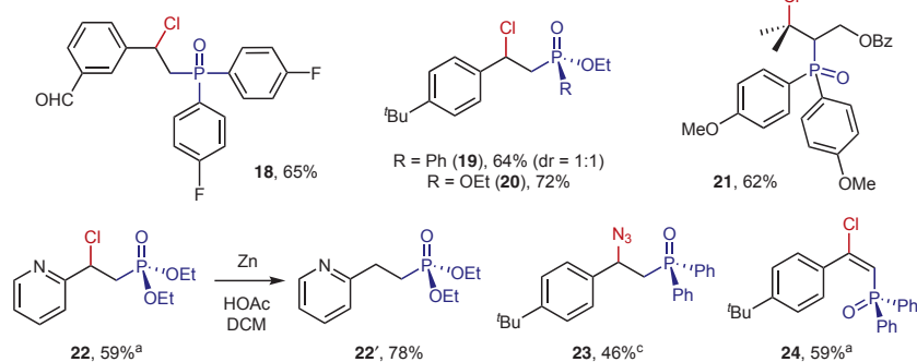
Scheme 2 Substrate scope. Reactions are conducted on 0.2 mmol scale under optimal conditions (see Table 1, entry 1); 10 isolated yields are reported.
