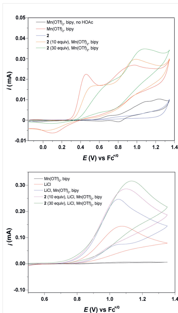
Figure 1 Cyclic voltammetry (CV) data. Top panel: characterization of the Mn catalytic complex in the absence or presence of acetate. Bottom panel: catalytic effect of Mn in the generation of Cl and P radical equivalents. Medium: 0.1 M LiClO_4 in HOAc/MeCN, unless otherwise noted in the figure; scan rate = 100 mV/s. See the Supporting Information for detailed conditions and full CV plots
