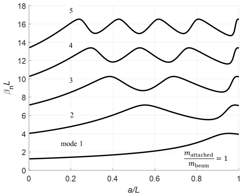
Figure 6. Eigenvalues of first 5 modes, \frac{m_{\text{attached}}}{m_{\text{beam}}} = 1 .
