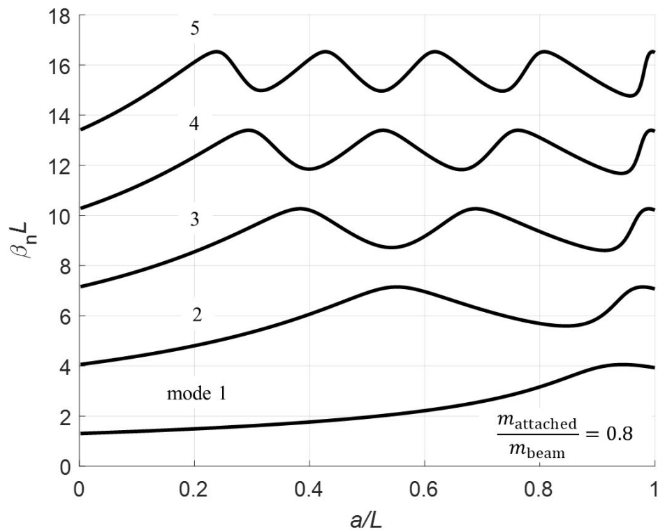
Figure 5. Eigenvalues of first 5 modes, \frac{m_{\text{attached}}}{m_{\text{beam}}} = 0.8 .
