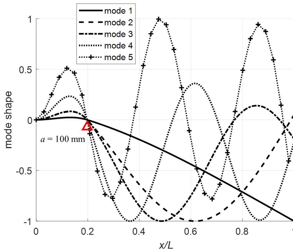
Figure 7. Mode shapes for pinned at a = 100 mm and \frac{m_{\text{attached}}}{m_{\text{beam}}} = 0.2 .
