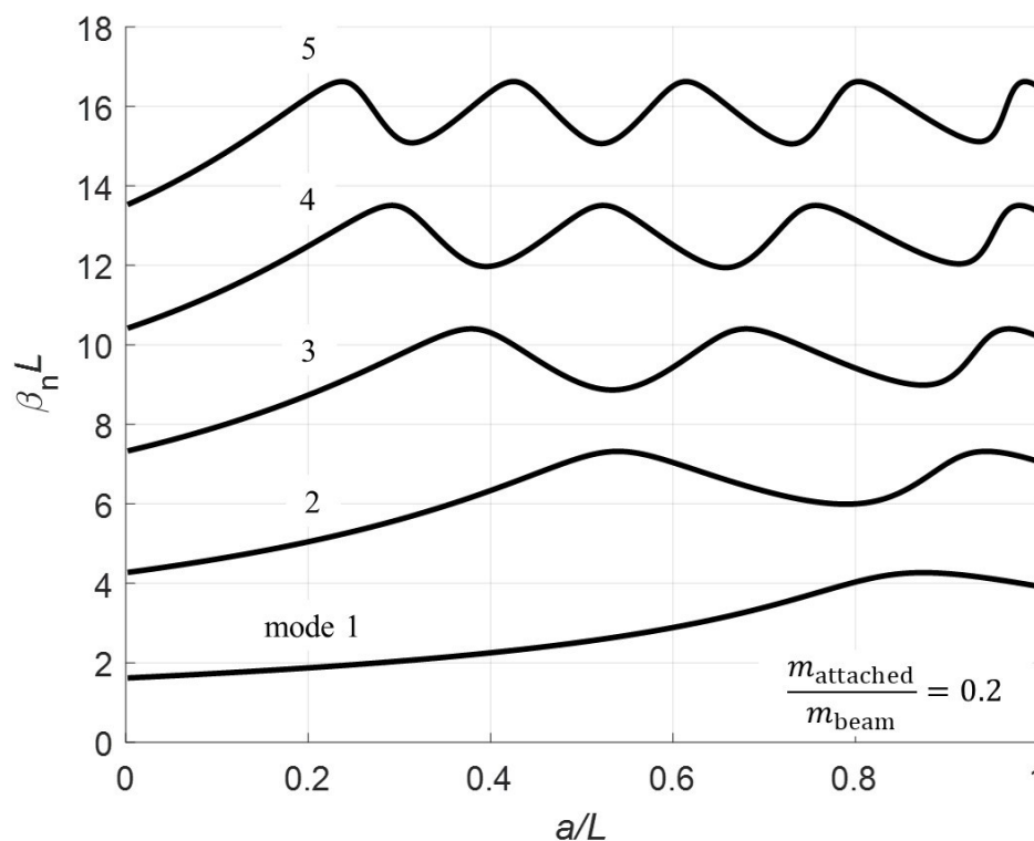
Figure 2. Eigenvalues of first 5 modes, \frac{m_{\text{attached}}}{m_{\text{beam}}} = 0.2 .
