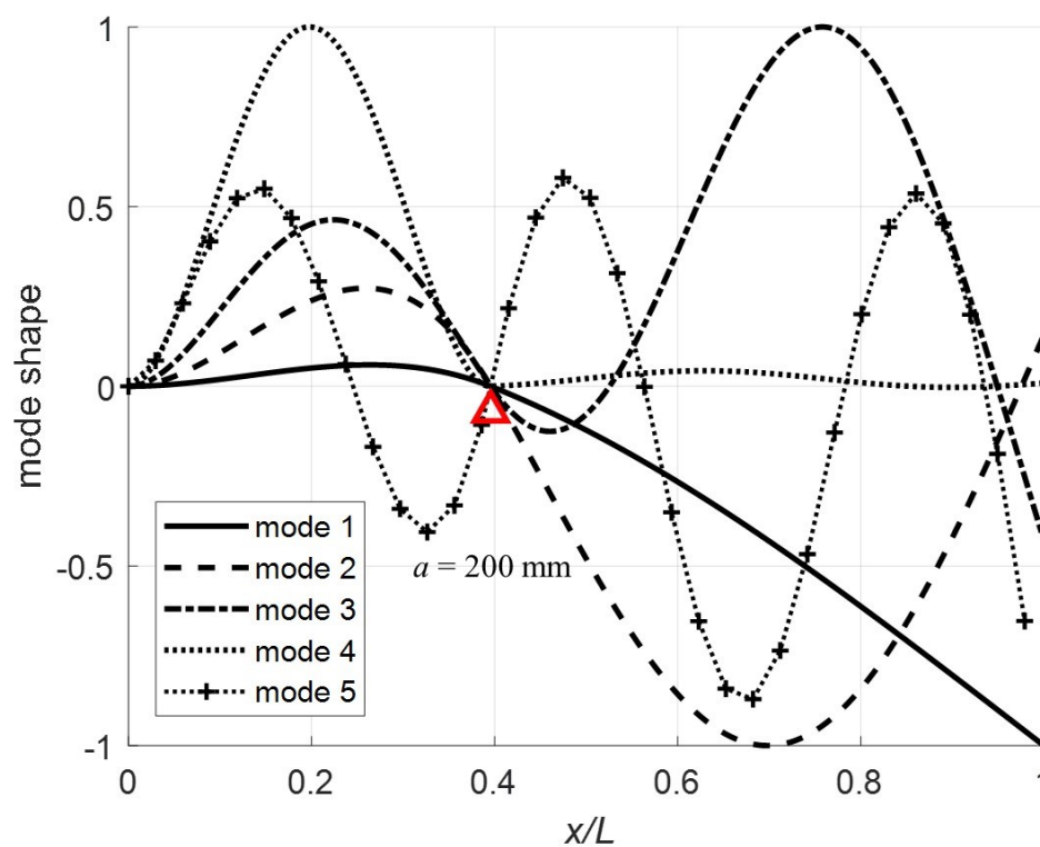
Figure 8. Mode shapes for pinned at a = 200 mm and \frac{m_{\text{attached}}}{m_{\text{beam}}} = 0.2 .
