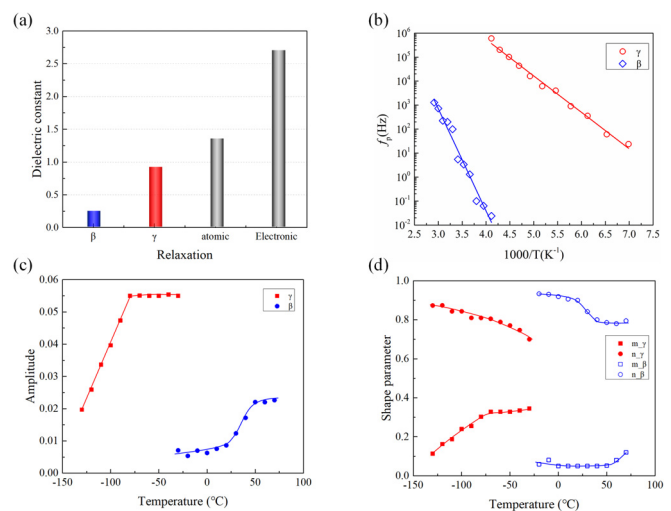
FIG. 3. (a) Contributions of different relaxation mechanisms to the dielectric constant. Atomic and electronic relaxation can be found in Ref. 18 in more detail. (b) Arrhenius plot of the characteristic frequency of the \beta and \gamma relaxation; (c) the amplitude of the \beta and \gamma relaxation as a function of temperature; and (d) the shape parameters m and n of \beta and \gamma relaxations.
