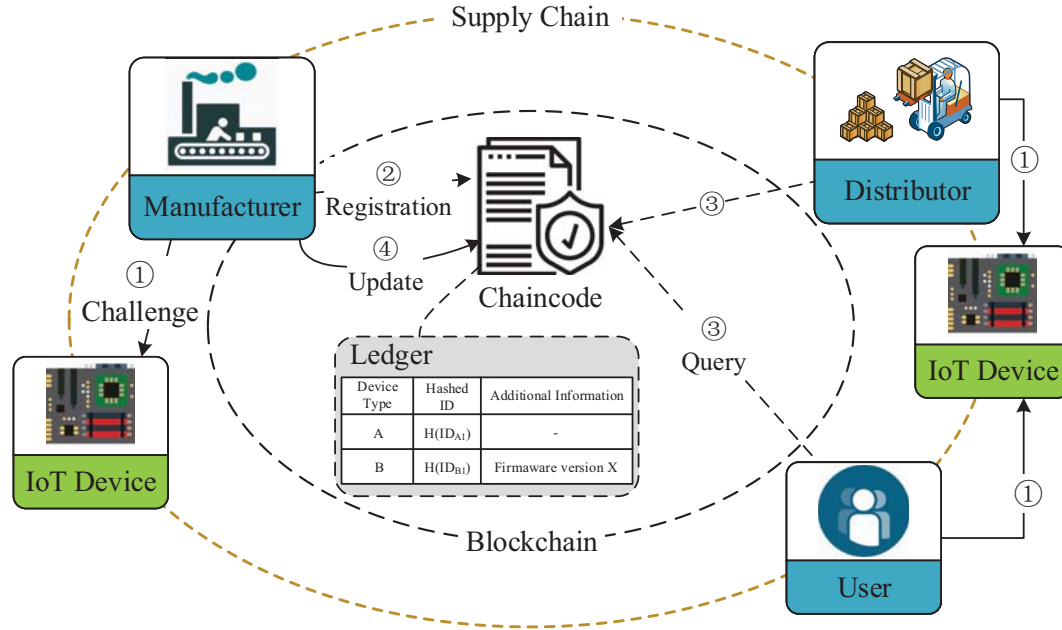
Figure 2: Proposed Blockchain based Authenticity Framework.
