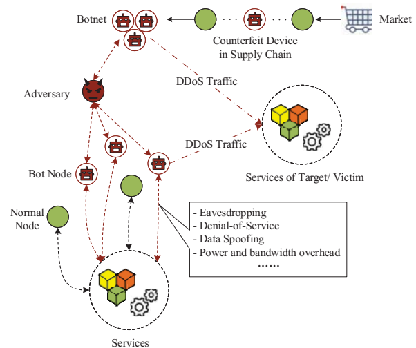
Figure 1: Threat model.
