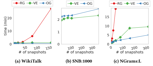
Figure 11: aZoom T : Fixed dataset size and group-by cardinality, varying number of snapshots. The number of nodes and edges is fixed to the largest graph size, and the group-by cardinality is fixed to the natural group-by cardinality of each dataset.
