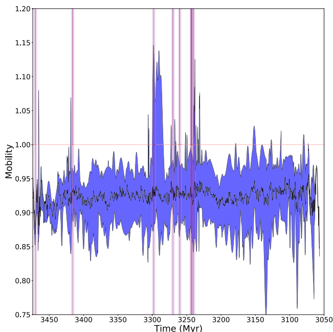
Figure 3. Evolution of mobility (ratio of internal root-mean-square velocities to those at surface) from all models over time. Exact age, size, velocity, and longitude of impacts S1–S8 (Table 1) are randomly selected from distribution based on uncertainties in these factors for each simulation (shown as purple vertical lines; mean age is darker purple, age uncertainty is lighter purple). Blue shaded area shows range of mobility demonstrated from all models throughout their evolution, as well as mean (thick black line) and maximum and minimum values (thin black lines). A number of runs had high mobility (and subduction) ca. 3.3–3.2 Ga. All models exhibited surface mobility values >1
