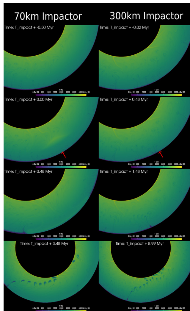
Figure 1. Series of modeled mantle temperature snapshots through time for a series of four impacts (S1–S4, from Johnson and Melosh, 2012; figures are shown from the time of impact S3 [T_impact = 3.243 Ga] onward), illustrating subduction initiation coincident with impact S3. Impactor sizes were held constant in this example, at either 300 km (to demonstrate effect of extreme example) or 70 km (maximum size of impactor S3 estimated from Johnson and Melosh [2012]). Red arrows show point of S3 impact. Ages of impacts are provided in Table 1.
