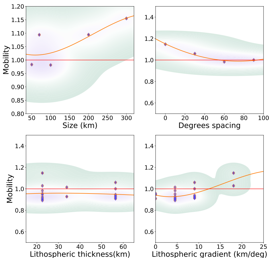
Figure 2. Modeled variation in mobility (ratio of internal root-mean-square velocities to those at surface) versus impact size (A), impact spacing (B; four impacts, either coincident or 30°, 60°, or 90° apart; impact ages as per Fig. 1), lithospheric thickness for a Monte Carlo spread of impact sizes based on uncertainties shown in Table 1 (so random velocities and longitude) (C), and lithospheric thickness gradient (averaged within a few degrees of impact) (D). Shaded regions are kernel density estimations (KDEs) of results (purple indicating high probability densities, green bracketing uncertainty projections).
