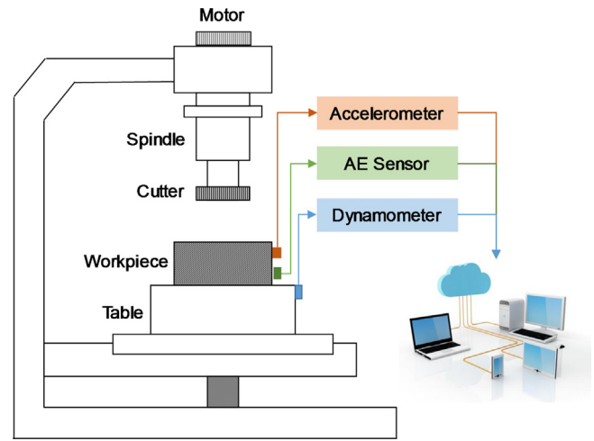
Fig. 10. Experimental Setup.
