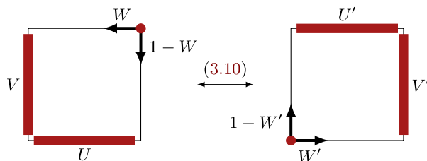
FIG. 3. Involution (3.10): Respectively, weights U and V on the south and west edges and west/south transition (W, 1 - W) become weights U' and V' on the north and east edges and east/north transition (W', 1 - W') , and vice versa.
