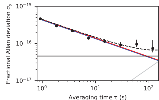
Fig. 4. Characterization of frequency stability.
