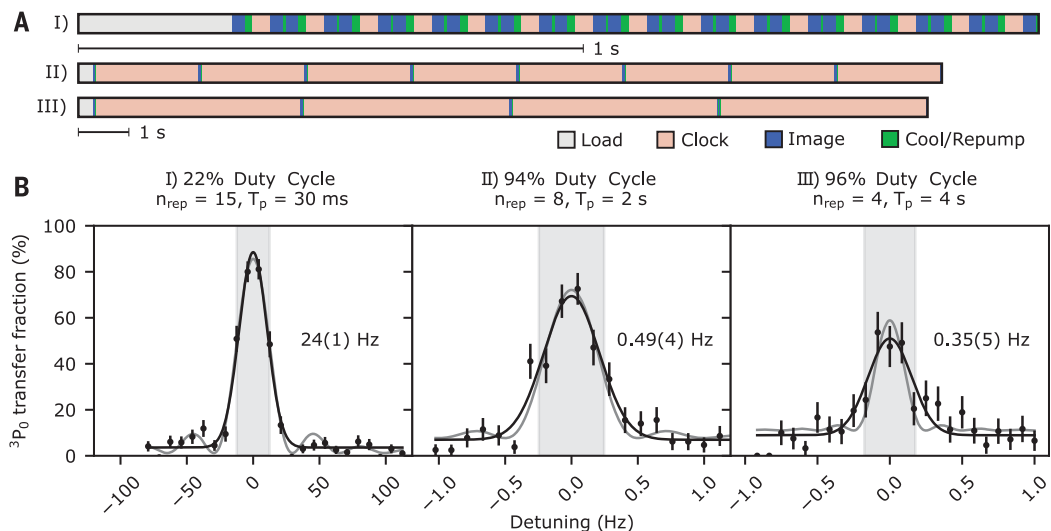
Fig. 3. Repeated nondestructive interrogation of the clock transition.
