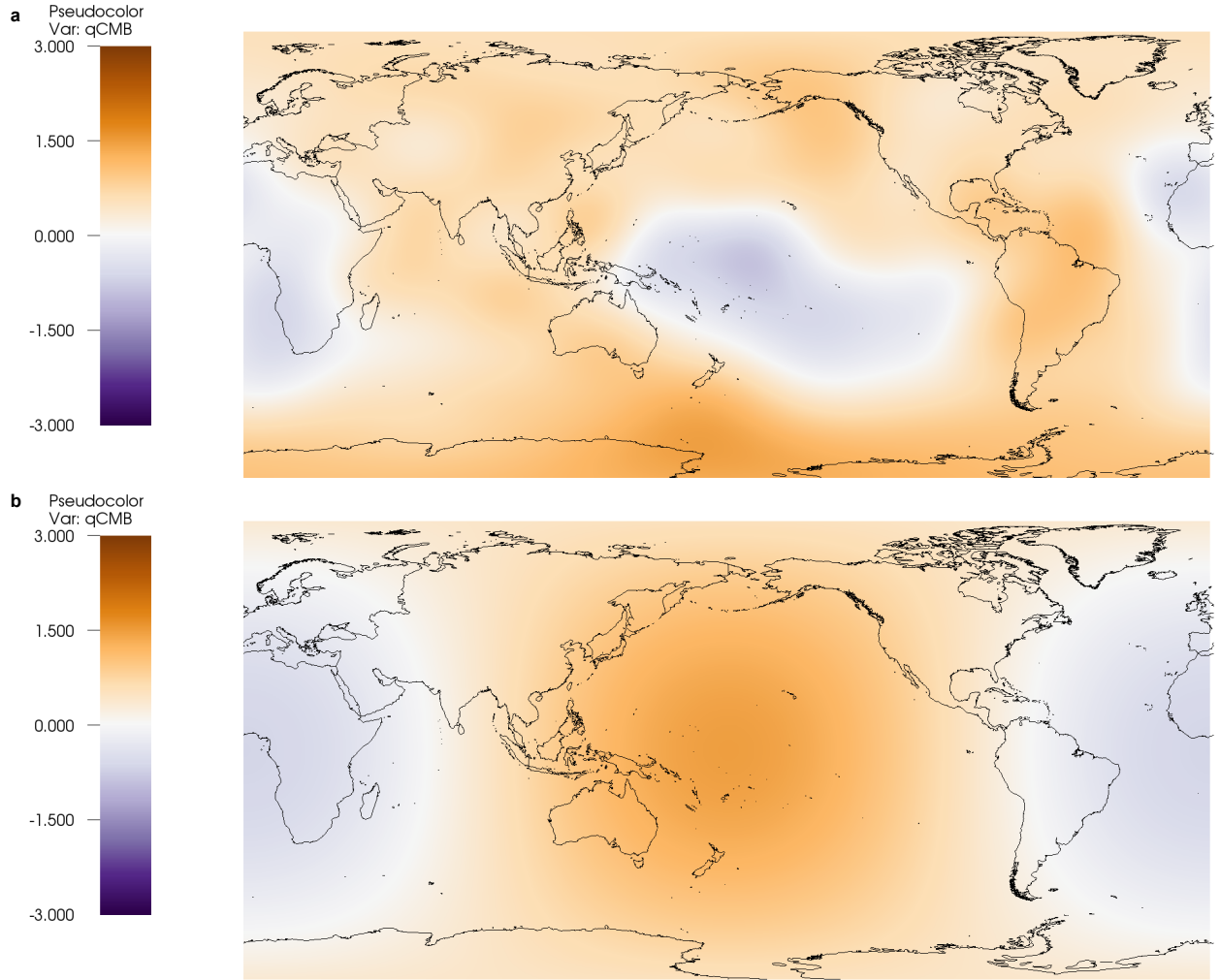
Figure 1: Patterns of CMB heat flux (nondimensional). a , tomographic pattern. b , hemispheric pattern. Both cases have q^* = 5.0 .
