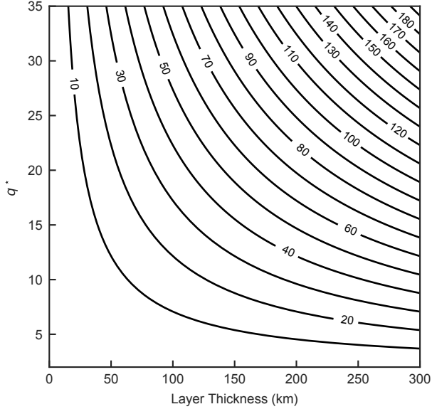
Figure 5: Excess temperature of the stratified regions. Contours of excess temperature (in kelvin) at the top of the core as a function of the layer thickness and the strength of heterogeneity, q^* . This example considers a total superadiabatic heat flow across the CMB of Q_{\text{conv}} = 0.6 TW, and thermal conductivity k = 100 \text{ W m}^{-1} \text{ K}^{-1} .
