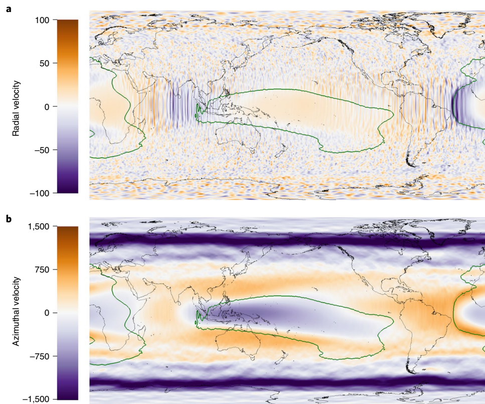
Fig. 4 | Flow -100 km below the CMB. a,b , Time-averaged radial velocity ( a ), azimuthal velocity ( b ) and contours of \partial T/\partial r=0 (green) for the simulation in Fig. 1. The averaging was done over 37 advection times. The flow velocity is non-dimensionalized as described in the Methods.
