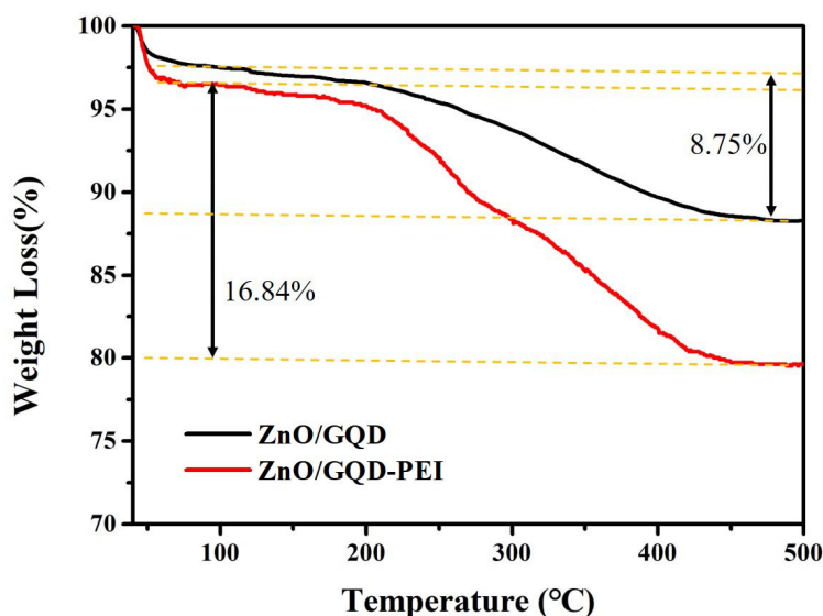
Figure 4. TGA curves of ZnO/GQD and ZnO/GQD-PEI(6×) nanocomposites.
