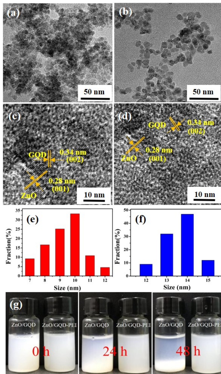
Figure 1. TEM images of (a,c) ZnO/GQD and (b,d) ZnO/GQD-PEI(6 \times ) nanocomposites, with the corresponding size distributions shown in panels (e) and (f), respectively. (g) Digital images of ZnO/GQD and ZnO/GQD-PEI(6 \times ) nanocomposites after different storage times.
