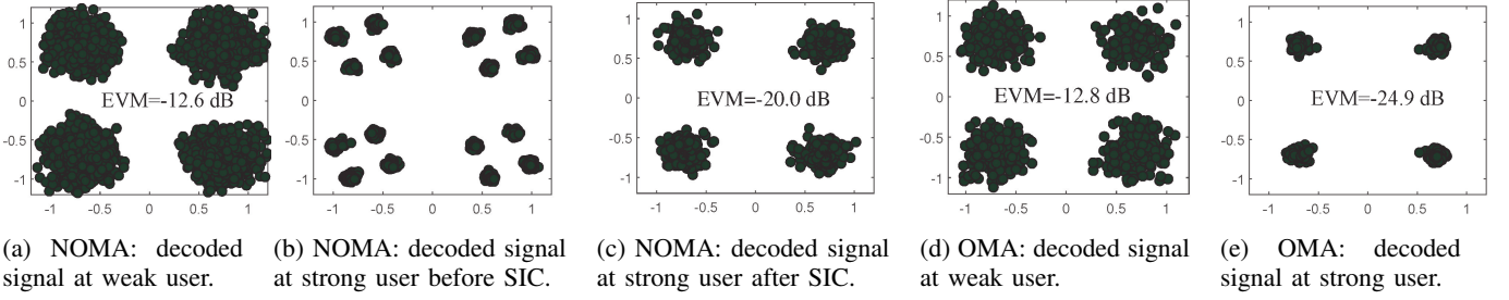
Fig. 11: Constellations of NOMA and OMA in downlink of WLAN where a two-antenna AP serves two single-antenna users.
