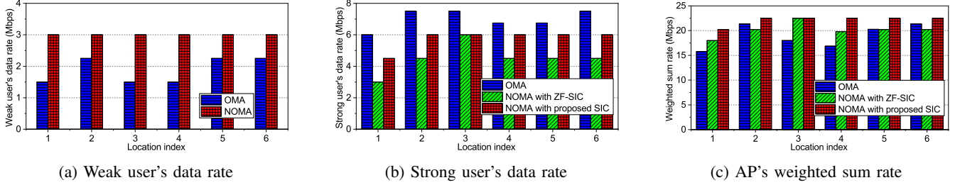
Fig. 10: Performance comparison of NOMA and OMA in downlink transmission of a WLAN where a single-antenna AP serves two single-antenna users.
