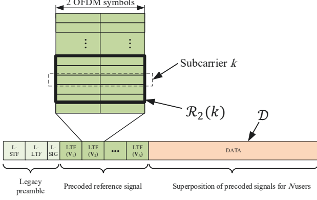
Fig. 7: Proposed frame structure for NOMA transmission.
