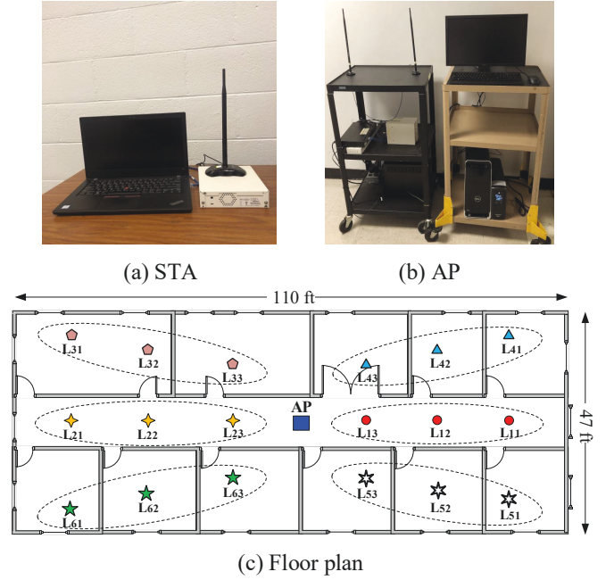
Fig. 8: Our NOMA testbed and floor plan.
