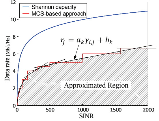
Fig. 3: The gap between Shannon capacity and the data rate achieved by MCS-based approach.
