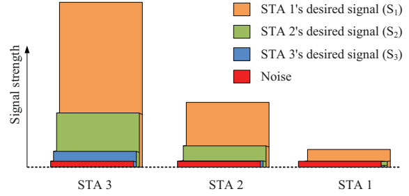
Fig. 2: Illustration of NOMA in downlink data transmission in a WLAN for N = 3 .
