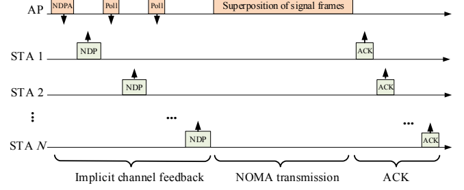
Fig. 6: A protocol for NOMA transmission in WLANs.
