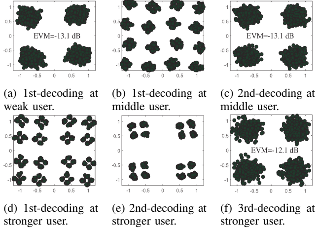
Fig. 13: Constellation of the decoded signals in downlink NOMA transmission when the two-antenna AP serves three single-antenna users.
