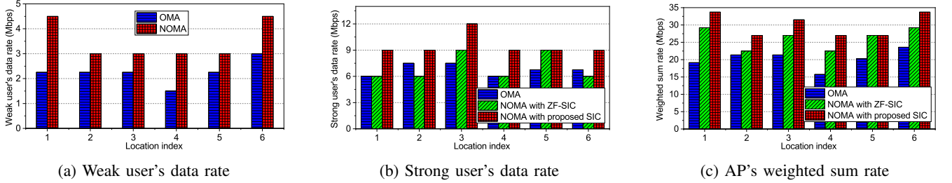
Fig. 12: Performance comparison of NOMA and OMA in downlink transmission of a WLAN where a two-antenna AP serves two single-antenna users.
