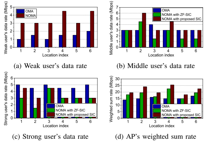
Fig. 14: Performance comparison of NOMA and OMA in downlink transmission when the two-antenna AP serves three single-antenna users.
