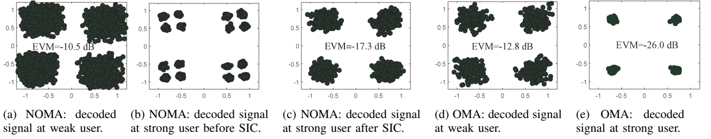
Fig. 9: Constellations of NOMA and OMA in downlink of WLAN where a single-antenna AP serves two single-antenna users.
