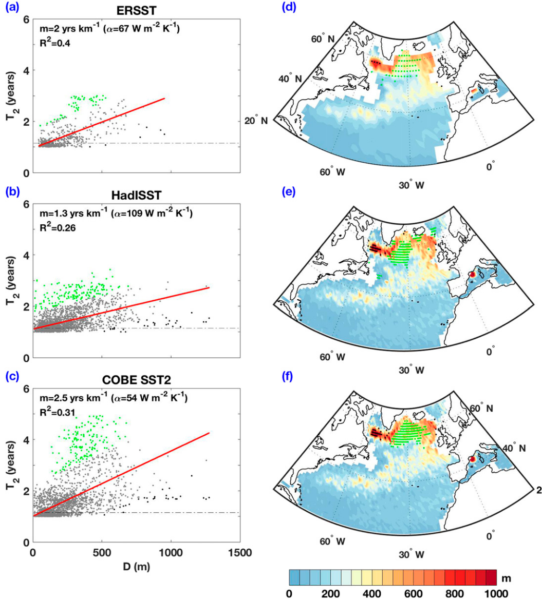
FIG. 8. How decorrelation time scales for wintertime SST are related to D : (left) Scatterplots comparing the decorrelation time scale T_2 for \text{SST}^w to D (from the Argo MLD product) for all points in the ETNA for (a) ERSST, (b) HadISST, and (c) COBE SST2. The dash-dotted gray lines show values of T_2 above which T_2 can be distinguished from white noise on interannual time scales (see the appendix ). The red line is a linear fit between T_2 and D , and the values of R^2 and the slope m and the corresponding value of the damping parameter \alpha [see Eq. (3)] are given in the top-left corner of each plot. Green (black) points are outliers that are more than two standard deviations above (below) the best fit line. (right) Spatial distribution of the outliers based on the linear fit for (d) ERSST, (e) HadISST, and (f) COBE SST2. Green (black) points are points more than two standard deviations above the best fit line, indicating points with higher (lower) than expected predictability. Colors show a spatial map of D from the Argo MLD product ( Holte et al. 2017 ).
