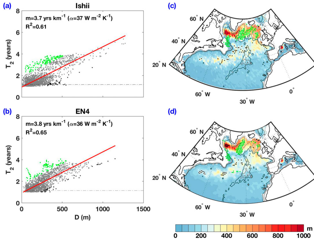
FIG. 7. Sensitivity of relationship between T_2 for H and D to the MLD product used: (a),(b) As in Figs. 6a and 6b and (c),(d) as in Figs. 6d and 6e, but D is from the Argo MLD climatology (Holte et al. 2017). This value of D is used for both the values of D in the scatterplot and in the calculation of H according to Eq. (1).
