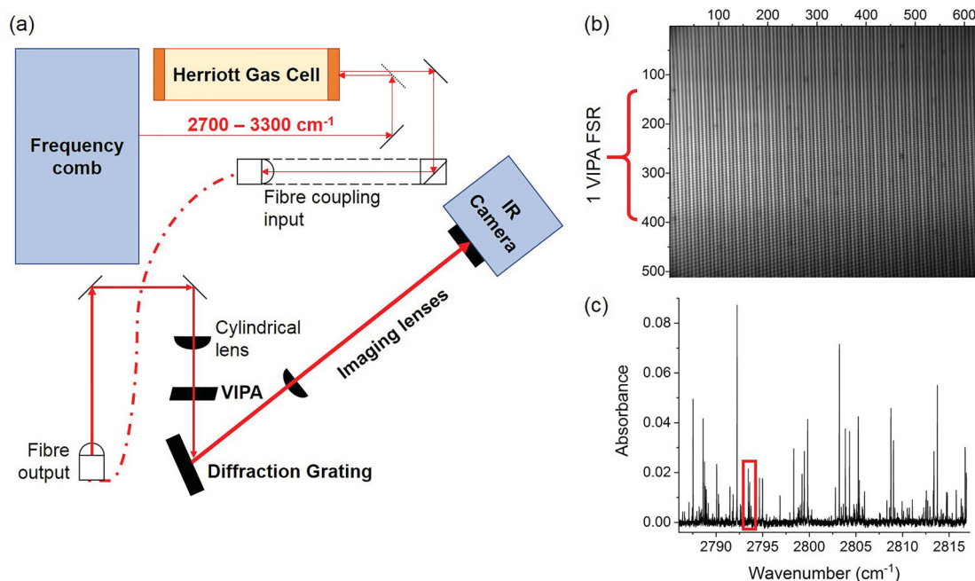
Figure 1. (a) Experimental setup, with important optical elements highlighted. (b) Greyscale image of a spatially dispersed f_{\text{rep}} = 250 MHz frequency comb on a 512 x 640 pixel InSb array camera, using a 50 \mu\text{s} exposure time and averaged for 190 images. Absorptions due to methane present in the gas cell (0.65% \text{CH}_4 in \text{N}_2 in 9.1 mbar total pressure) are seen as an attenuation of the light. The vertical spatial coverage of one VIPA FSR (51 comb teeth) is marked on the left. (c) Absorption spectrum resulting from interleaving 10 different f_{\text{rep}} images, one of which is panel (b). The red box indicates the region of the spectrum detailed in Fig. 3.
