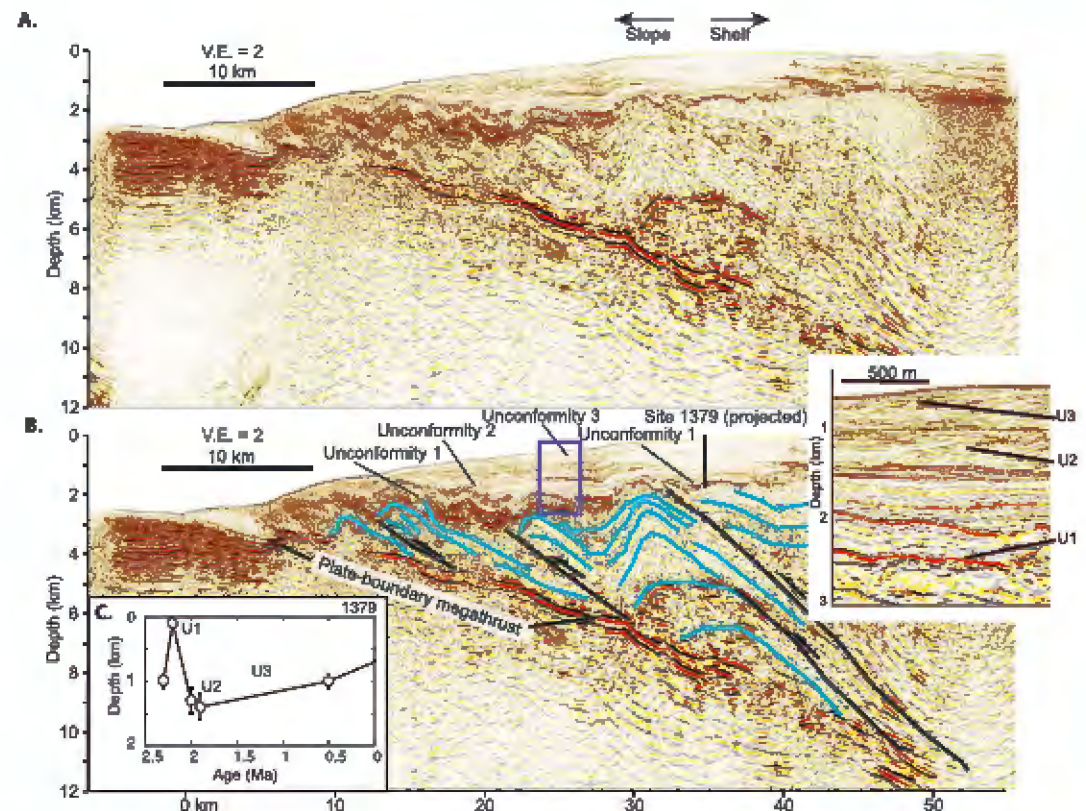
Figure 2. (a) Uninterpreted seismic section from the Costa Rica Seismogenesis Project (CRISP) 3-D volume, with location shown in Figure 1. V.E. denotes vertical exaggeration. (b) Interpreted section as in (a) showing location of unconformities, faults, and folds (Bangs et al., 2016; Edwards et al., 2018). Dark blue box shows location of blowup. (c) Uplift or subsidence data from core at Site 1379 after backstripping for the effects of sediment loading from Vannucchi et al. (2013). U1, U2, and U3 refer to unconformities 1, 2, and 3, respectively.
