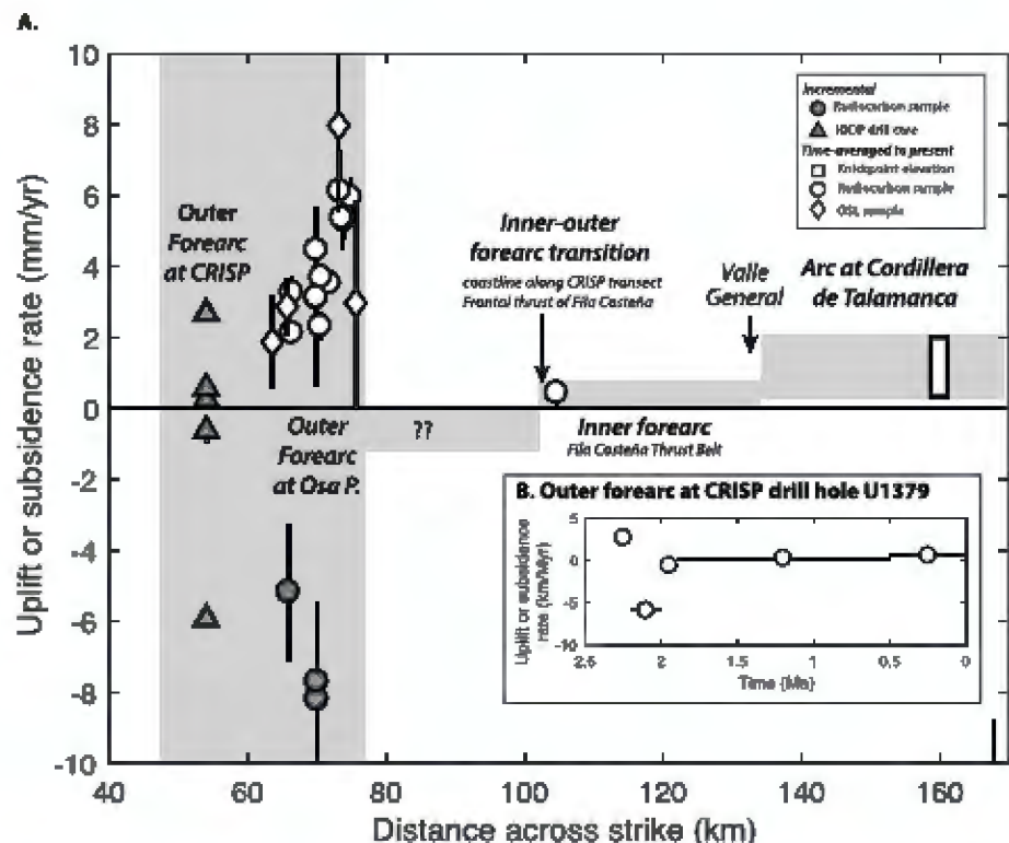
Figure 8. (a) Rock uplift (positive) or subsidence (negative) rates compiled from offshore and onshore regions near the CRISP transect. See Figure 3 for location of samples. Offshore data derived from paleodepth calculations and backstripping from ocean drilling at hole U1379 (Vannucchi et al., 2011), with age control from nanofossil analysis and benthic foraminifera distributions (Table 1; Vannucchi et al., 2013). Onshore data calculated from the elevation and ages of radiocarbon and optically stimulated luminescence (OSL) samples shown in Tables 2 and 3 with data from Gardner et al. (1992), Sak et al. (2004), Fisher et al. (2004), and Gardner et al. (2013). Ranges of rock uplift rates are reported for the Talamanca Range calculated from the elevation of 21 knickpoints relative to current base level, and an onset of increased rock uplift starting at 1, 2, or 3 Ma (Morell et al., 2012). (b) Calculated incremental uplift or subsidence rates based on data from Vannucchi et al. (2013) and Vannucchi, Morgan, Silver, et al. (2016) from data shown in Table 1. CRISP = Costa Rica Seismogenesis Project; IODP = Integrated Ocean Drilling Program.
