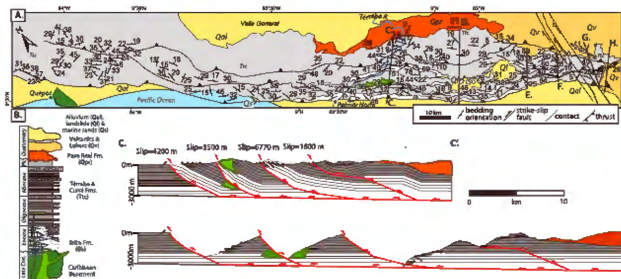
Figure 5. (a) Geologic map of the Fila Costeña Thrust Belt, showing ~75 new bedding orientation data combined with previously published data from Fisher et al. (2004), Sitchler et al. (2007), Morell et al. (2008), Sak et al. (2009), Morell et al. (2013), and Morell (2016). The décollement beneath the Fila Costeña steps up section in the northwestern portion of the thrust belt and therefore does not expose the Brito Fm. Thrust locations in this northwestern region are therefore mapped based on field observations of fault contacts and projected along strike parallel to the topographic grain. (b) Stratigraphic column of the Central Fila Costeña Thrust Belt showing units displayed in (a), modified from Phillips (1983) and Fisher et al. (2004). The Brito Fm. is ~1 km thick. (c) New balanced cross section based on data following the Térraba River (see location in panel a). Cross section constructed by forward modeling to match mapped contacts, thrust traces, and surface structural measurements in 2-D Move. The cross section was constructed taking into account both the dip measurements shown, as well as data from the regional mapped structure, which suggests that thrust faults do not change orientation significantly along strike and on average dip consistently to the northeast by 15–35°.
