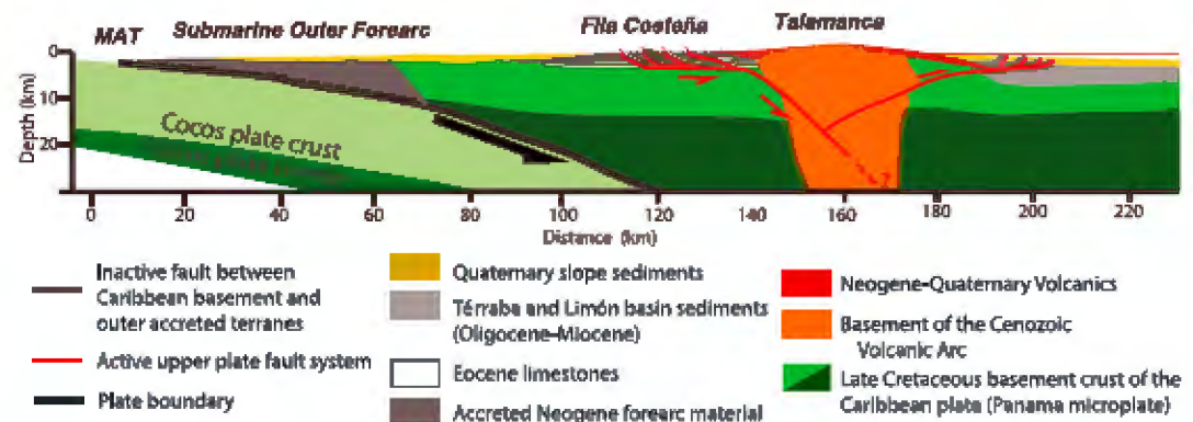
Figure 4. Cross section of the Costa Rican forearc-arc-backarc system along transect in Figure 3 (labeled as “xsn”) based on Stavenhagen et al. (1998), Hayes et al. (2012), Buchs et al. (2009), Fisher et al. (2004), Brandes et al. (2007), and Morell et al. (2012).
