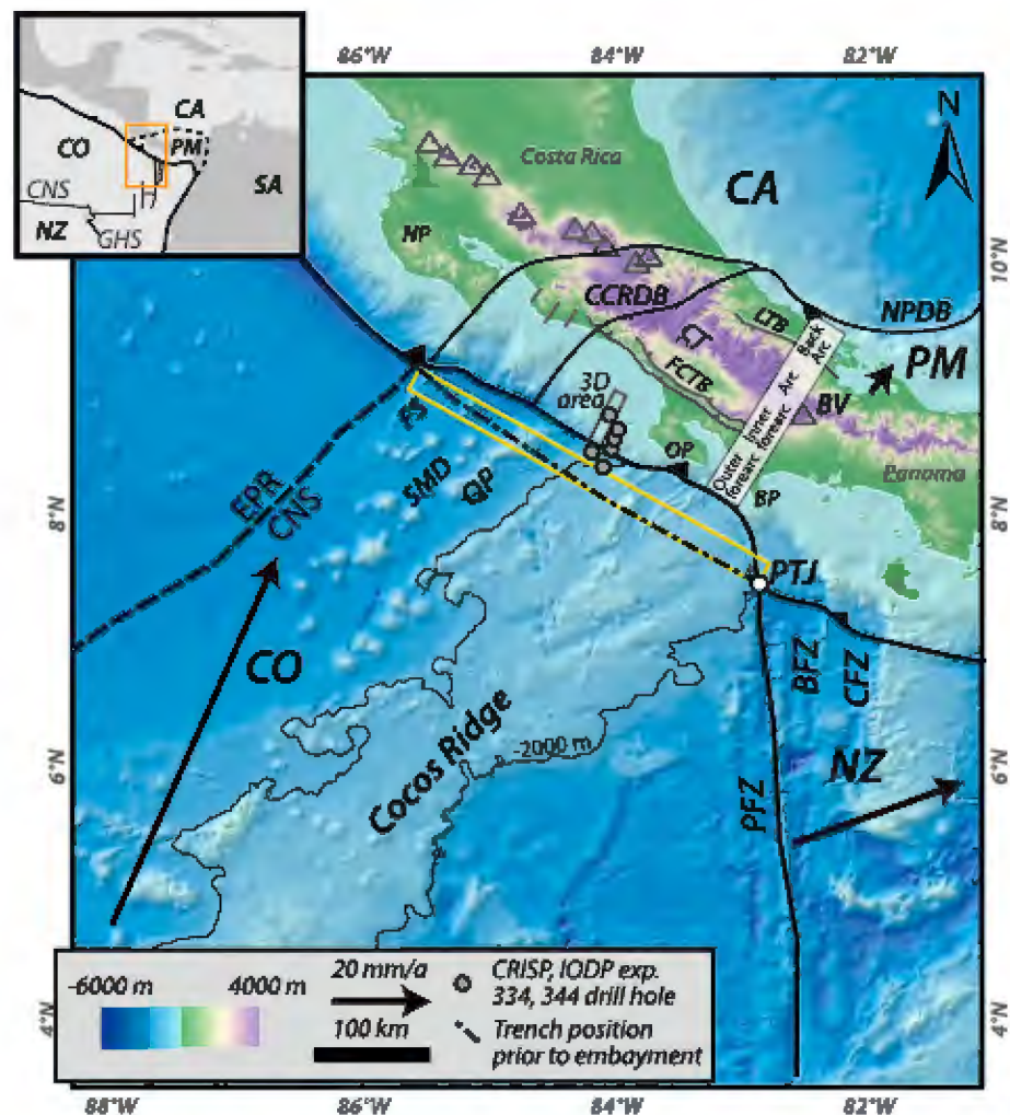
Figure 1. Regional tectonic setting of the southern Costa Rica subduction zone. Costa Rica Seismogenesis Project (CRISP) 3-D seismic area denoted by “3-D area” box. Black arrows show plate motion relative to stable Caribbean plate (CA; Argus et al., 2011; DeMets, 2001; Kobayashi et al., 2014). Dash-dotted line shows former position of the trench following Vannucchi et al. (2013). Yellow box shows bathymetry swath and location of crustal thickness data from Walther (2003) as shown in Figure 7. Triangles show currently active volcanoes. Large-scale tectonic features compiled from Silver et al. (1990), Kolarsky et al. (1995), Fisher et al. (1998), Marshall et al. (2000), Barckhausen et al. (2001), Fisher et al. (2004), Sitchler et al. (2007), and Brandes et al. (2007). BFZ, Balboa Fracture Zone; BP, Burica Peninsula; BV, Barú Volcano; CCRDB, Central Costa Rica Deformed Belt; CNS, Cocos-Nazca Spreading Center; CO, Cocos plate; CFZ, Coiba Fracture Zone; CT, Cordillera de Talamanca; EPR, East Pacific Rise; FCTB, Fila Costeña Thrust Belt; FS, Fisher Seamount; GHS, Galápagos Hot Spot; LTB, Limón Thrust Belt; NP, Nicoya Peninsula; NPDB, North Panama Deformed Belt; NZ, Nazca Plate; OP, Osa Peninsula; PM, Panama microplate; PTJ, Panama Triple Junction; QP, Quepos Plateau; SA, South America Plate; SMD, Seamount domain. Bathymetry from GEBCO (General Bathymetric Chart of the Oceans) and Ranero et al. (2003). Topography from the National Aeronautics and Space Administration’s Shuttle Radar Topography Mission 90-m data set and GTOPO-30.
