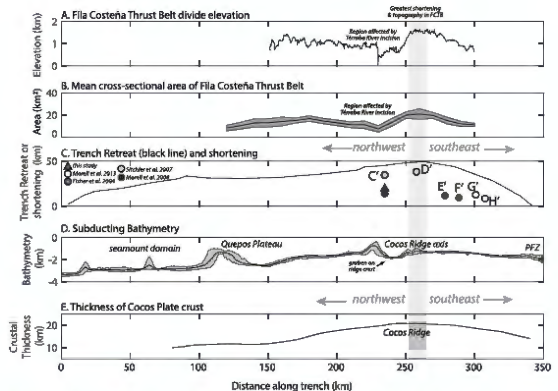
Figure 7. (a) Elevation of the Fila Costeña Thrust Belt (FCTB) drainage divide from data in Figure 6. (b) Mean cross-sectional area of Fila Costeña Thrust Belt relative to current sea level and 1\sigma uncertainty within 10-km-wide and 30-km-long swaths as shown in Figure 6. Topographic analysis based on SRTM-30-m data. (c) Trench retreat estimated following Vannucchi et al. (2013) as the distance between the present-day trench and the assumed projection shown as dash-dotted line in Figures 1 and 3. Shortening estimates across the Fila Costeña from cross sections as shown in Figure 5 (denoted as C–H) are derived from this study, Fisher et al. (2004), Sitchler et al. (2007), Morell et al. (2008), and Morell et al. (2013). Total shortening amounts along cross sections E' and F' from Morell et al. (2008) are somewhat lower than adjacent cross sections because they do not include slip along the rearmost thrust due to insufficient structural data in this region. (d) Mean, maximum, and minimum bathymetry along swath shown in Figure 1 from Ranero et al. (2003) relative to mean sea level. PFZ denotes Panama Fracture Zone. (e) Thickness of Cocos plate crust on incoming plate along profile line shown in Figure 1 (Sallarès et al., 1999; Walther, 2003).
