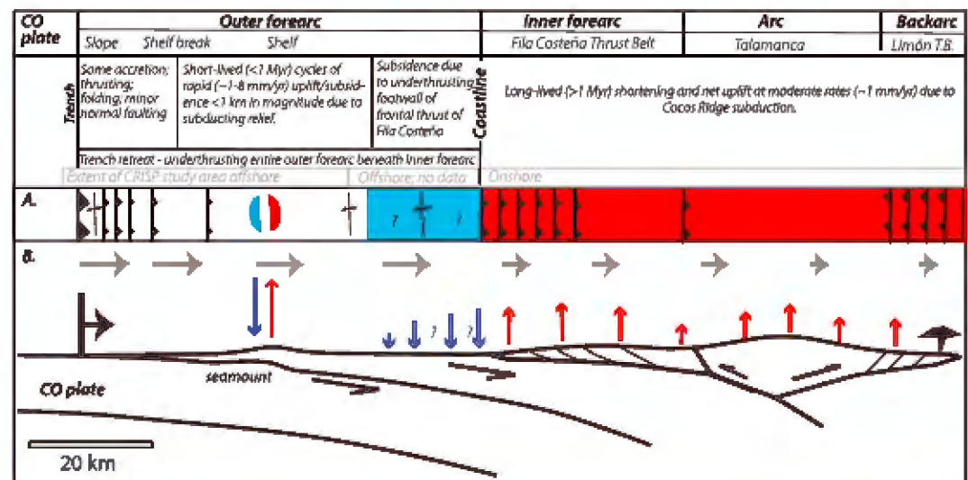
Figure 9. Cartoon showing proposed model for the Quaternary evolution of the outer forearc of southern Costa Rica along the CRISP transect. Panel (a) shows map view cartoon depiction of uplift (red) or subsidence (blue) along the transect. Panel (b) shows locations of relative rates of uplift (red arrows) or subsidence (blue arrows) at positions along the transect. Gray arrows show relative movement of the forearc toward a pinned backarc. Vertical scale is exaggerated to highlight important features and is not to scale. The coastline demarcates a dichotomy in vertical tectonics between the offshore forearc and the inner forearc-arc-backarc system. The submarine forearc records: (1) yo-yo tectonics and sharp reversals between periods of rapid subsidence and uplift that last less than ~1 Myr (Vannucchi et al., 2013; Vannucchi, Morgan, Silver, et al., 2016) as a consequence of subducting bathymetric relief, similar to results from the Osa Peninsula (Gardner et al., 2013; Sak et al., 2004). The onland inner forearc-backarc system records: (1) telescoping of the forearc (Fisher et al., 2004; Morell et al., 2008, 2013; Sitchler et al., 2007) and backarc (Brandes et al., 2007; Silver et al., 1990) basins and (2) long-term uplift across the inner forearc at the Fila Costeña (Fisher et al., 1998, 2004; Sak et al., 2009), volcanic arc at the Cordillera de Talamanca (Morell et al., 2012), and the backarc at the Limón backarc thrust belt (Limón T.B.; Brandes et al., 2007) due to Cocos Ridge subduction. CO indicates Cocos plate. CRISP = Costa Rica Seismogenesis Project.
