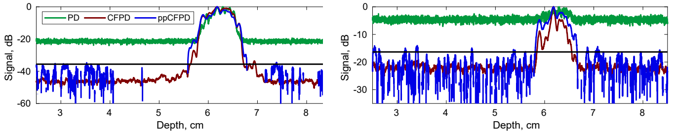
Fig. 7: Axial cross sections of simulation data for 10dB channel SNR ( left ) and -10dB channel SNR ( right ) cases. Realization shown depicts a 100% fractional moving blood volume case. The black line depicts the theoretical threshold.
