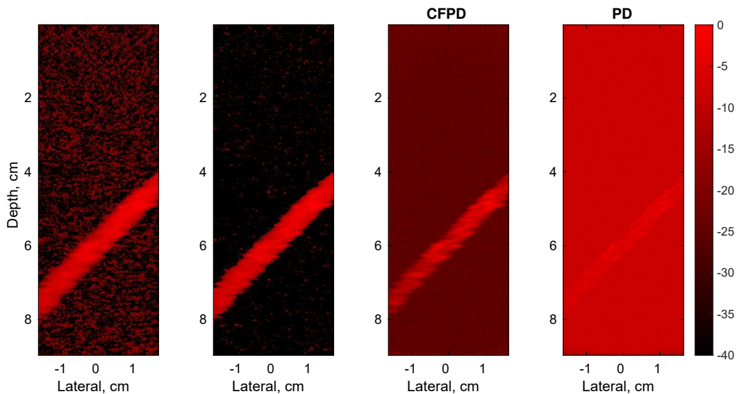
Fig. 1: Comparison of image formation techniques. For ppCFPD, application of the theoretical threshold (ppCFPD, adaptive) suppressed the noise floor more effectively than thresholding negative values (ppCFPD, zero). Note that the dynamic range is extended so that the noise floor is visible in all cases. Images depict a 100% fractional moving blood volume realization with -10dB blood channel SNR.
