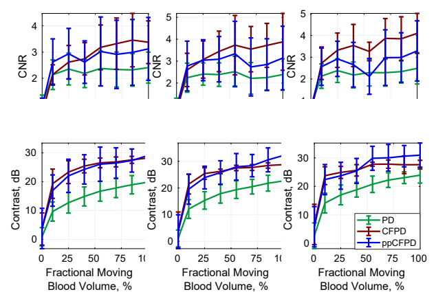
Fig. 12: CNR and Contrast plots for phantom data obtained at 11, 16, and 21 V. Mean and standard deviation of metrics shown for the 5 cm/s velocity realizations.
