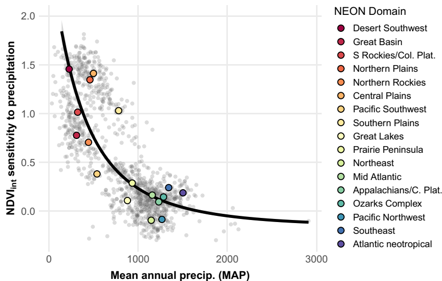
Figure 2 Sensitivity of primary production (NDVI int ) to precipitation derived from a mixed-effects model relating the two variables at USHCN stations from years 2000 through 2015 (model P -value for annual precipitation < 0.001). The y-axis units represent the change in annual primary production (NDVI int ) per meter of change in precipitation. The sensitivity values of individual USHCN stations (fixed + domain random + station random effects) are shown as grey points and the sensitivity values of NEON domains (fixed + domain random effects) are shown as coloured points (see Fig. S1 for reference). A nonlinear model fit to individual station sensitivities is shown in black ( NDVI_{int} : prcp = c * (e^{-MAP}) , Efron's R^2 = 0.52 , P < 0.001 ).
