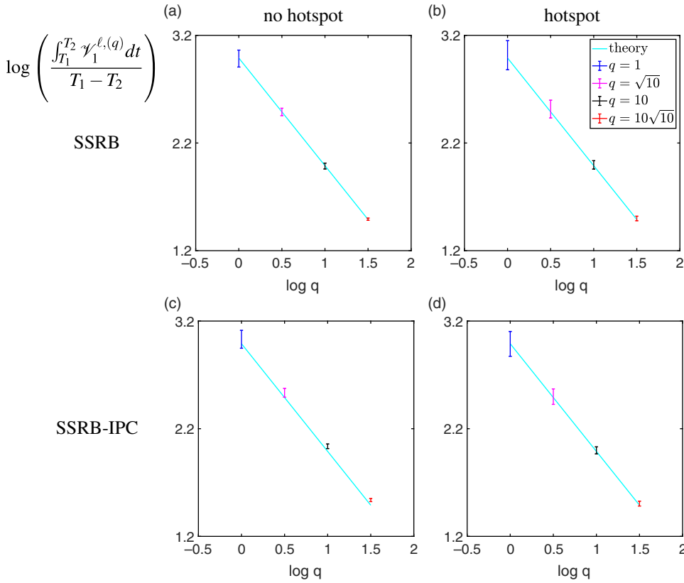
FIGURE 11. Comparison of the log–log plot of the theoretical and true scaling in (3.32) with error bars for both zero hotspot formation and hotspot formation. The straight lines show the theoretical scaling with slope -1 and the x -intercept \ell^2 \Theta^2 \mathfrak{d} |\phi^\ell|_2^2 \cong 2.9892 , where \mathfrak{d} = 0.019 , \Theta = 5.6 , and \phi^\ell is assumed as in 3.30. The error bars show the true scaling, with [T_1, T_2] set as [0, 10] , [1, 11] , [2, 12] , ..., [719, 729] , [720, 730] . For the SSRB model [104], (a) shows results with no hotspot, and the error bars with x -axis as 0, 1, 2 and 3 show results with the simulations of the blue, magenta, black and red lines in Figure 10 (a), respectively. (b) shows results with hotspot formation, and the error bars with x -axis as 0, 1, 2 and 3 show results with the simulations of the blue, magenta, black and red lines in Figure 10 (b), respectively. For the SSRB-IPC model, (c) shows results with no hotspot, and the error bars with x -axis as 0, 1, 2, and 3 show results with the simulations of the blue, magenta, black and red lines in Figure 10 (c), respectively. (d) shows results with hotspot formation, and the error bars with x -axis as 0, 1, 2 and 3 show results with the simulations of the blue, magenta, black and red lines in Figure 10 (d), respectively.
