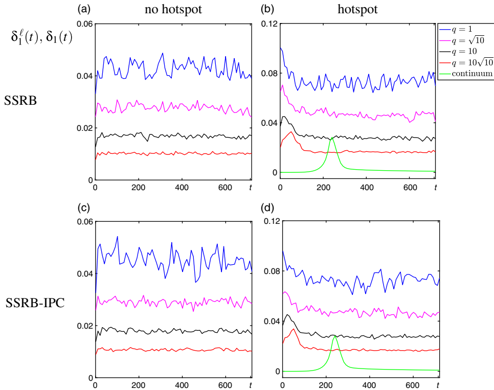
FIGURE 7. Examples of the L^1 -area rate of change \delta_1^\ell(t) and \delta_1(t) for SSRB and SSRB-IPC models for zero hotspot formation and hotspot formation. For the SSRB model [104], (a) shows results with cases of zero hotspot formation, and the blue, magenta, black and red lines represent the statistics of the models plotted in Figures 1(a), (b), 2(a) and (b), respectively. (b) shows results associated with the hotspot formation regimes, and the blue, magenta, black, red and green lines show results with the simulations in Figures 3(a), (b), 4(a), (b) and 5, respectively. For the SSRB-IPC model, (c) shows results with cases of zero hotspot formation, and the blue, magenta, black and red lines represent the statistics of the models plotted in Figures 1(c), (d), 2(c) and (d), respectively. (d) shows results associated with the hotspot formation regimes, and the blue, magenta, black, red and green lines show results with the simulations in Figures 3(c), (d), 4(c), (d) and 5, respectively.
