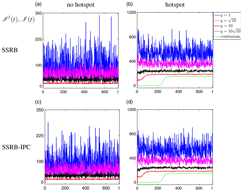
FIGURE 6. Examples of the relative Fisher information \mathcal{J}^\ell(t) and \mathcal{J}(t) for zero hotspot formation and hotspot formation. For the SSRB model [104], (a) shows results with cases of zero hotspot formation, and the blue, magenta, black and red lines represent the statistics of the models plotted in Figures 1(a), (b), 2(a) and (b), respectively. (b) shows results associated with the hotspot formation regimes, and the blue, magenta, black, red and green lines show results with the simulations in Figures 3(a), (b), 4(a), (b) and 5, respectively. For the SSRB-IPC model, (c) shows results with cases of zero hotspot formation, and the blue, magenta, black and red lines represent the statistics of the models plotted in Figures 1(c), (d), 2(c) and (d), respectively. (d) shows results associated with the hotspot formation regimes, and the blue, magenta, black, red and green lines show results with the simulations in Figures 3(c), (d), 4(c), (d) and 5, respectively.
