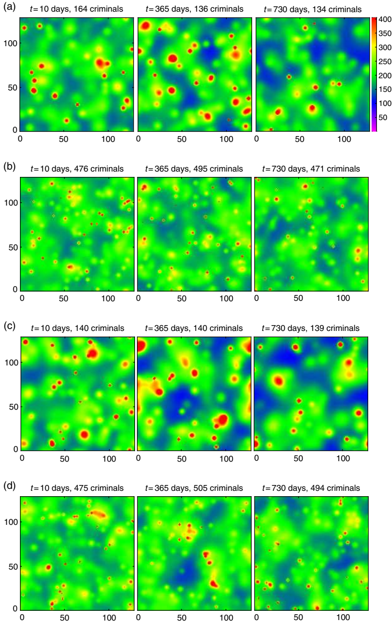
FIGURE 1. Plot of the attractiveness A_s^\ell(t) for the SSRB model [104] and the SSRB-IPC model. For both models, the initial conditions (at t = 0 ) and parameters are set as A_0 = 1/30 , B_0^\ell \equiv \bar{B} , n_0^\ell \cong \bar{n}^\ell , D = 100 , L = 128 , \ell = 1 , \omega = 1/15 , and \eta = 0.2 . For the SSRB model [104], in (a) and (b), we set \Gamma = 0.0019q , \theta = 5.6/q , q = 1 in (a), and q = \sqrt{10} in (b). For the SSRB-IPC model, in (c) and (d), we set \Gamma = 0.0019q , \theta = 5.6/q , q = 1 in (c), and q = \sqrt{10} in (d). (a) and (c) show the dynamic hotspot regimes, while (b) and (d) show less degree of transience of hotspots.
