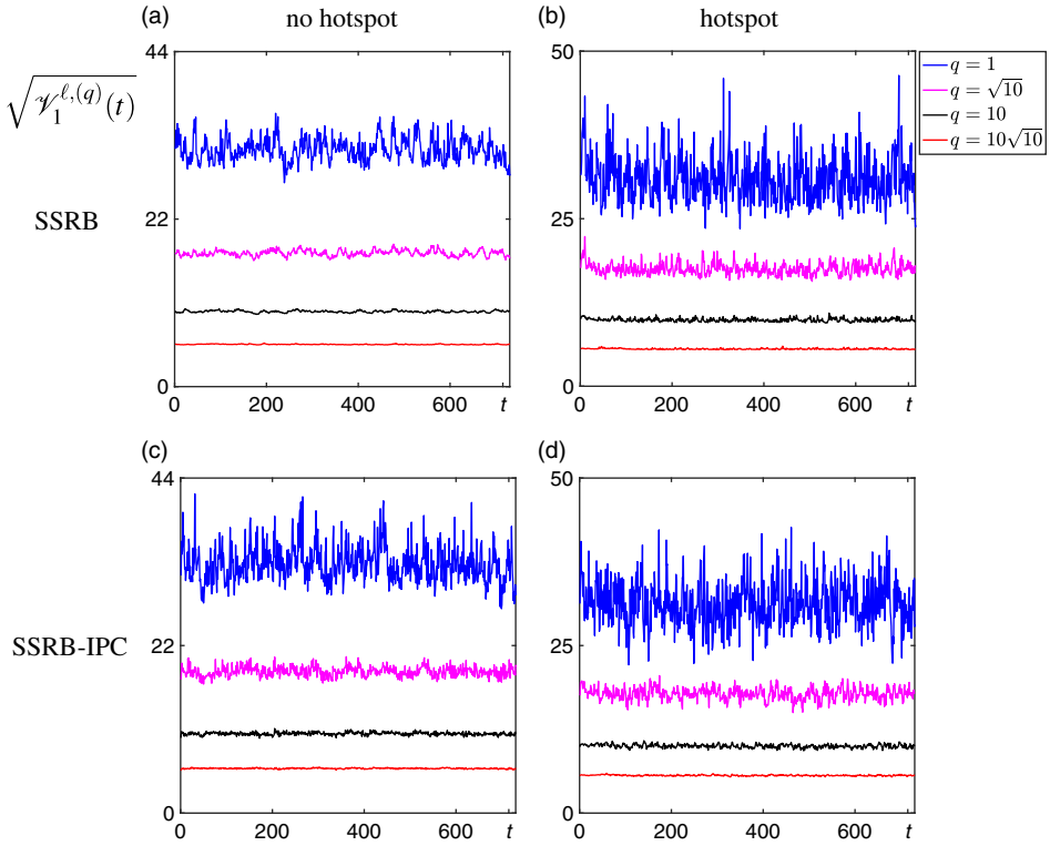
FIGURE 10. Examples of the infinitesimal standard deviation for attractiveness, \sqrt{\gamma_1^{\ell, (q)}(t)} , in the cases of zero hotspot formation and hotspot formation. For the SSRB model [104], (a) shows results in the cases with no hotspot. The blue, magenta, black and red lines show results with the simulations in Figures 1(a), (b), 2(a) and (b), respectively. (b) shows results with hotspot formation. The blue, magenta, black and red lines represent results with the simulations in Figs 3(a), 3(b), 4(a) and 4(b), respectively. For the SSRB-IPC model, (c) shows results in the cases with no hotspot. The blue, magenta, black and red lines show results with the simulations in Figures 1(c), (d), 2(c) and (d), respectively. (d) shows results with hotspot formation. The blue, magenta, black and red lines represent results with the simulations in Figs 3(c), 3(d), 4(c) and 4(d), respectively.
