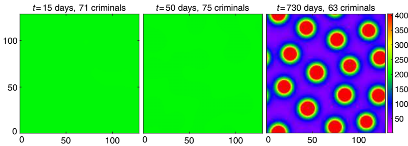
FIGURE 5. Output of the attractiveness A(\mathbf{x}, t) for the continuum analogue of the SSRB model with hotspot formation. The parameters and data are the equivalent of those used to create plots in Figures 3 (a)–(d) and 4 (a)–(d).
