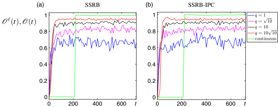
FIGURE 8. Examples of the relative overlapping area, \mathcal{O}^\ell(t) and \mathcal{O}(t) , associated with hotspot formation regimes. For the SSRB model [104], in (a), the blue, magenta, black, red and green lines represent the statistics of the models plotted in Figures 3(a), (b), 4(a), (b) and 5, respectively. For the SSRB-IPC model, in (b), the blue, magenta, black, red and green lines show results with the simulations in Figures 3(a), (b), 4(a), (b) and 5, respectively.
