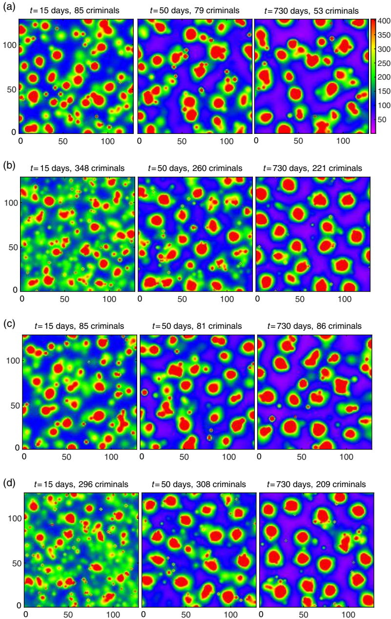
FIGURE 3. Plot of the attractiveness A_s^\ell(t) for the SSRB model [104] and the SSRB-IPC model. For both models, the parameters and initial conditions (at t = 0 ) are set as L = 128 , \ell = 1 , D = 100 , \omega = 1/15 , \eta = 0.03 , A_0 = 1/30 , n_0^\ell \cong \bar{n}^\ell , and B_0^\ell is set to be \bar{B} except for sites with slight perturbations. For the SSRB model [104], in (a) and (b), we set \Gamma = 0.0019q , \theta = 5.6/q , q = 1 in (a), and q = \sqrt{10} in (b). For the SSRB-IPC model, in (c) and (d), we set \Gamma = 0.0019q , \theta = 5.6/q , q = 1 in (c), and q = \sqrt{10} in (d). (a) and (c) show the dynamic hotspot regimes, while (b) and (d) show less degree of transience of hotspots.
