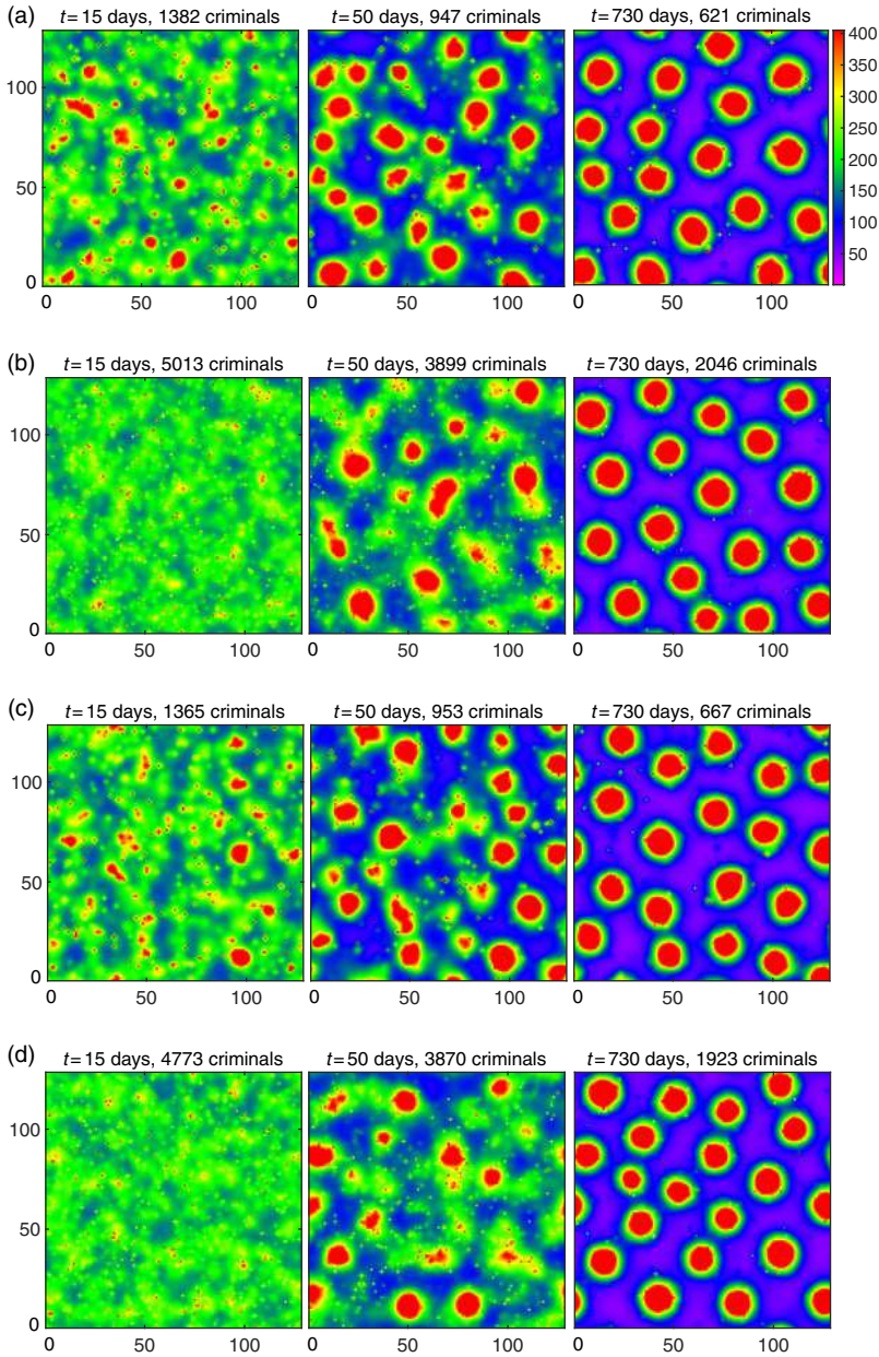
FIGURE 4. Plot of the attractiveness A_s^\ell(t) for the SSRB model [104] and the SSRB-IPC model. For both models, the parameters and initial conditions (at t = 0 ) are set as L = 128 , \ell = 1 , D = 100 , \omega = 1/15 , \eta = 0.03 , A_0 = 1/30 , n_0^\ell \cong \bar{n}^\ell , and B_0^\ell is set to be \bar{B} except for sites with slight perturbations. For the SSRB model [104], in (a) and (b), we set \Gamma = 0.0019q , \theta = 5.6/q , q = 10 in (a), and q = 10\sqrt{10} in (b). For the SSRB-IPC model, in (c) and (d), we set \Gamma = 0.0019q , \theta = 5.6/q , q = 10 in (c), and q = 10\sqrt{10} in (d). (a) and (c) show the stationary hotspots regimes. (b) and (d) show even less degree of transience of hotspots.
