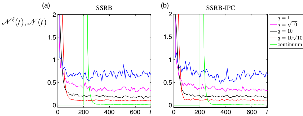
FIGURE 9. Examples of the relative non-overlapping area, \mathcal{N}^\ell(t) and \mathcal{N}(t) , associated with hotspot formation regimes. For the SSRB model [104], in (a), the blue, magenta, black, red and green lines represent the statistics of the models plotted in Figures 3(a), (b), 4(a), (b) and 5, respectively. For the SSRB-IPC model, in (b), the blue, magenta, black, red and green lines show results with the simulations in Figures 3(a), (b), 4(a), (b) and 5, respectively.
