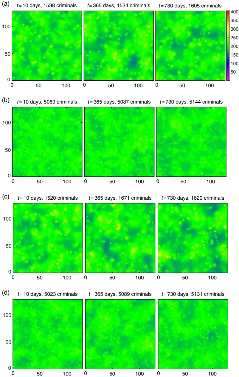
FIGURE 2. Plot of the attractiveness A_s^\ell(t) for the SSRB model [104] and the SSRB-IPC model. For both models, the initial conditions (at t = 0 ) and parameters are set as A0 = 1/30 , B0_s^\ell \equiv \bar{B} , n0_s^\ell \cong \bar{n}^\ell , D = 100 , L = 128 , \ell = 1 , \omega = 1/15 and \eta = 0.2 . For the SSRB model [104], in (a) and (b), we set \Gamma = 0.0019q , \theta = 5.6/q , q = 10 in (a), and q = 10\sqrt{10} in (b). For the SSRB-IPC model, in (c) and (d), we set \Gamma = 0.0019q , \theta = 5.6/q , q = 10 in (c), and q = 10\sqrt{10} in (d). (a) and (c) show the spatially homogeneous regimes, and (b) and (d) show even less transience of hotspots.
