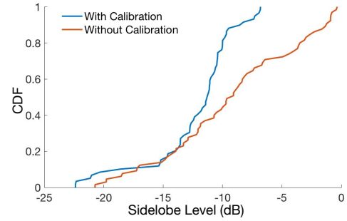
Fig. 8. Performance of Calibration. CDF of sidelobe level relative to the main beam with and without calibration. The figure shows that calibration significantly reduces the radiation outside of the main beam.
