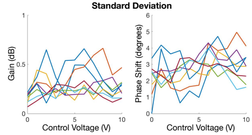
Fig. 7. Stability of Calibration. Standard deviation of calibration result. The figure shows that the calibration is stable within 1dB gain deviation and 5 degree phase deviation.
