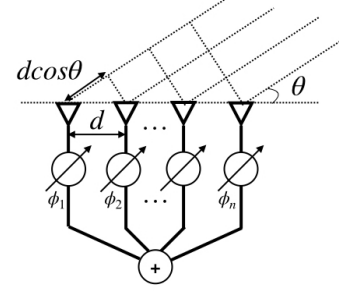
Fig. 2. Phased Array System. Phased array system can steer a beam at a direction \theta by shifting the phase of signals.
