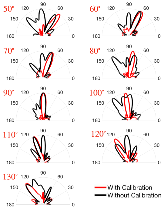
Fig. 9. Beam Patterns. The measured beam patterns steered at 9 different angles are shown. The beam patterns before (black) and after (red) calibration are compared. The peak magnitude is normalized for better visualization.
