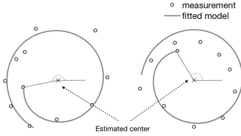
Fig. 5. Measured Channel Estimation and Model. The figure shows the channel estimation from two phase shifters with the fitted model. The relative phase can be evaluated by comparing the reference state.
