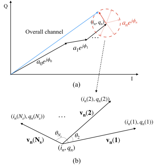
Fig. 3. Channel Estimation Constellation. (a) Each phase shifter contributes to the overall channel response. (b) The response of phase shifter is determined by a given model. Changing the control state of the phase shifter will move the channel response.
