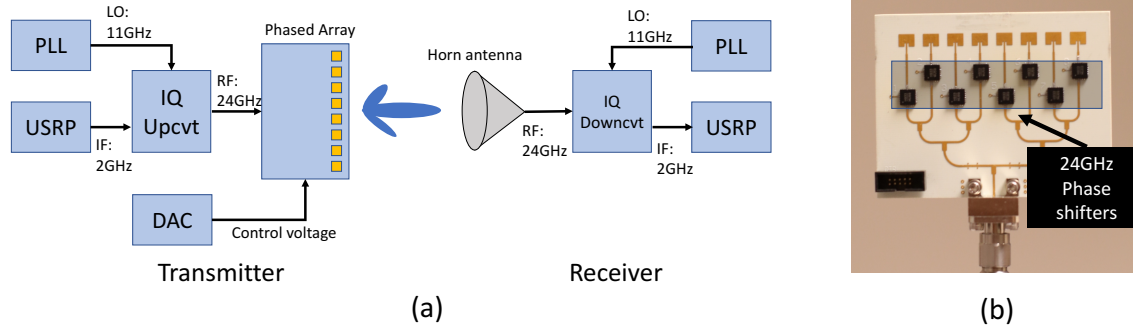
Fig. 4. Hardware Block Diagram and Phased Array. (a) Block diagram of the mmWave transmitter and receiver system we built. (b) The 8-element phased array. Each 24GHz phase shifter is connected to a patch antenna. The control voltage is provided by an external DAC through the connector.
