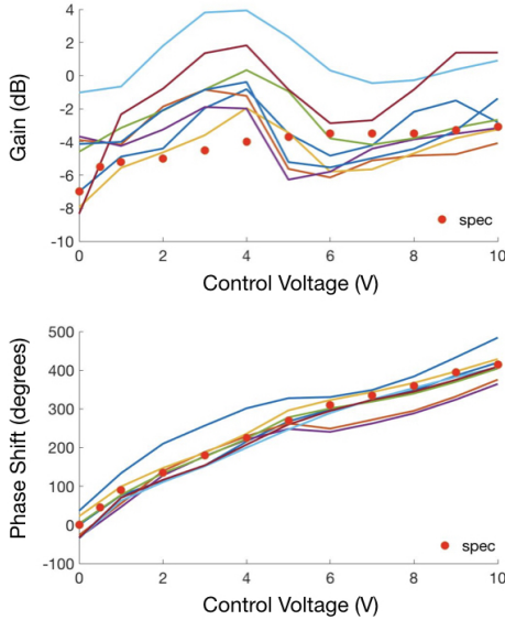
Fig. 6. Estimated Gain and Phase. The figure shows the estimated gain and phase of the 8 phase shifters over the control voltage. The red dots shows the specification of the phase shifter.
