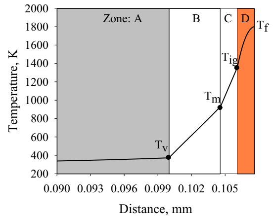
Fig. 7. Detailed flame structure obtained via numerical solution of the 1D flame propagation problem, clearly showing the different zones and their thicknesses.
