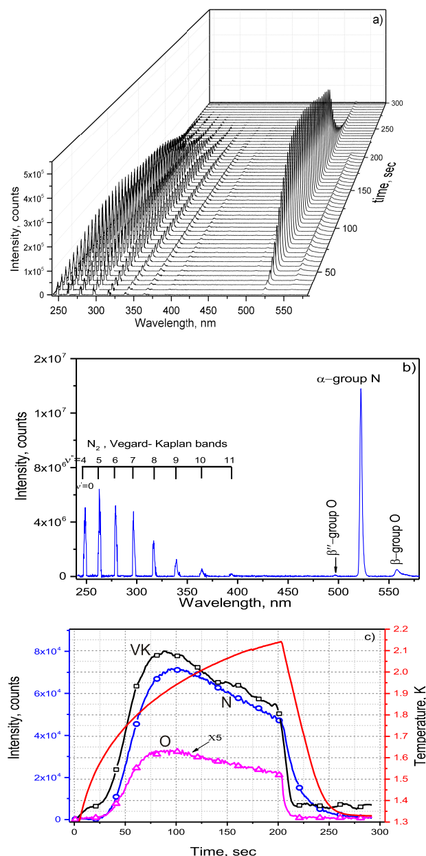
Fig. 2. (Color online) Thermoluminescence of ensemble of nitrogen–argon nanoclusters immersed in superfluid helium. An ensemble of nanoclusters was prepared from gas mixture [\text{N}_2]/[\text{Ar}]/[\text{He}] = 1/1/200 . (a) Dynamics of thermoluminescence spectra of the ensemble of nanoclusters during warming up from 1.3 to 2.15 K. Each spectrum in the figure is a sum of 100 spectra taken with exposure time 50 ms. (b) Integrated thermoluminescence spectra obtained during entire warming process. (c) Time dependence of sample temperature (red line). Time dependences of thermoluminescence intensity for nitrogen molecules integrated over all observed VK bands (black line with squares), nitrogen atoms (blue line with circles) and oxygen atoms (magenta line with triangles).
