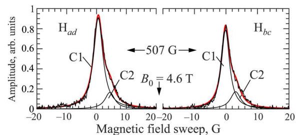
FIG. 6. The ESR spectra of H atoms in HD film.
