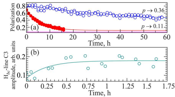
FIG. 4. (a) Relaxation of H atom nuclear polarization after applying the Overhauser effect DNP in as-deposited H_2 Sample 1 (open blue circles) and HD sample (red circles) measured at T=0.8 K. H atom nuclear polarization at T=0.8 K according to Boltzmann statistics is shown by a solid magenta line. Note the large difference in the T_{1N} times for H_2 and HD samples. The solid blue and red lines were obtained by fitting the experimental data by the formula p(t) = p + a \exp(-t/T_{1N}) . (b) Amplitude of the H_{bc} -line C3 component after applying the Overhauser effect DNP measured in as-deposited H_2 Sample 2 at T=0.9 K. The dark cyan line was obtained by fitting the experimental data by the formula A(t) = A + a \exp(-t/T_{1N}) where A is the H_{bc} ESR line amplitude.
