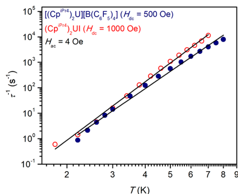
Figure 6. Plot of the relaxation rate ( \tau^{-1} ) versus temperature ( T ) (log–log scale) for polycrystalline samples of (\text{Cp}^{\text{Ir}4})_2\text{UI} ( 1 ) and [(\text{Cp}^{\text{Ir}4})_2\text{U}][\text{B}(\text{C}_6\text{F}_5)_4] ( 5 ). Relaxation times for 1 were extracted from ac susceptibility measurements between 1.8 and 7.0 K, while those for 5 were extracted from measurements between 2.2 and 8.0 K. The red and blue circles represent the measured relaxation rates for 1 and 5 , respectively, while the black solid lines correspond to the best fit of the relaxation times according to the equation \tau^{-1} = CT^n .
