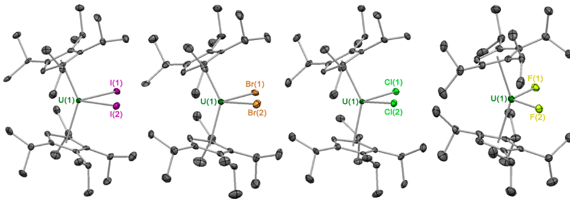
Figure 1. X-ray crystal structures of (\text{Cp}^{\text{iPr}_4})_2\text{UX}_2 ( 2-X ) with 50% probability ellipsoids. From left to right, 2-I , 2-Br , 2-Cl , and 2-F are shown. Hydrogen atoms are omitted for clarity. Selected structural metrics are listed in Table 1.
