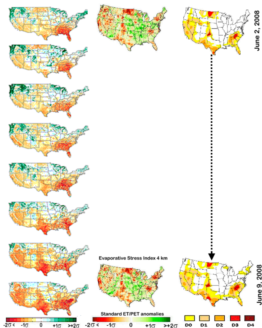
Figure 8. An example of daily proxy ESI with the integrated MODIS and AMSR-E LST input (the first column), as compared with the current ESI (the second column), and the weekly US Drought Monitor (USDM) drought map (the third column).
