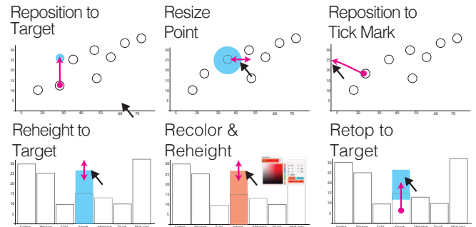
Fig. 6. Strategies to navigate a data point over time.
