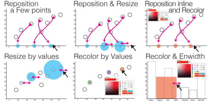
Fig. 4. Prominent strategies to assign a data attribute to an axis (first row); and to the size or color of points in the scatterplot, and of bars in the bar chart (second row).
