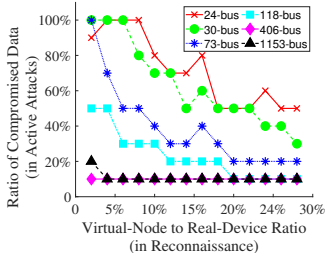
Fig. 13: Virtual nodes vs. compromised data when FN rate is less or equal to 0.5%.
