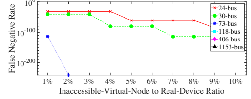
Fig. 21: False negative rate of the probabilistic dropping protocol with \delta = 4 and p_0 = 0.18 .
