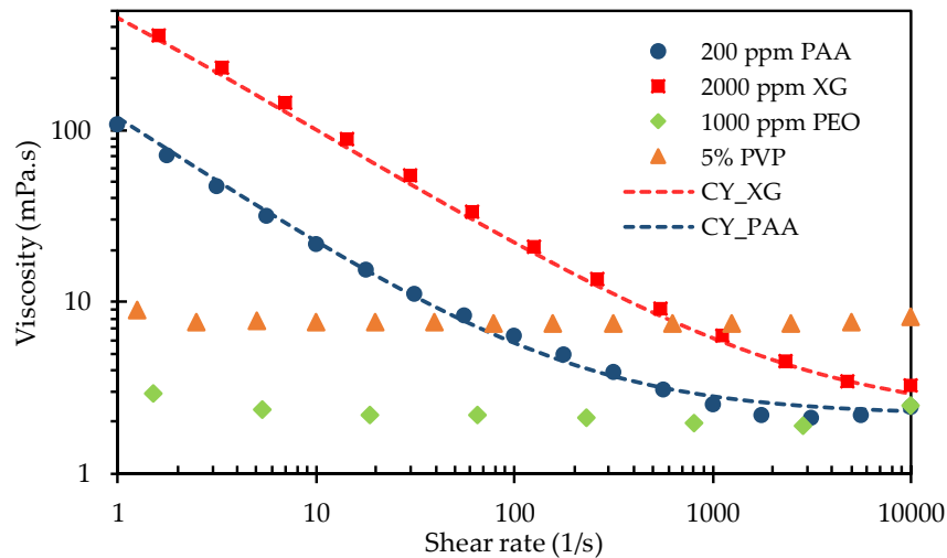
Figure 2. Experimentally measured viscosity data (symbols) of the prepared non-Newtonian fluids, where the dotted lines show the curve-fitting for the two shear-thinning xanthan gum (XG) and polyacrylamide (PAA) solutions using the Carreau–Yasuda model.
