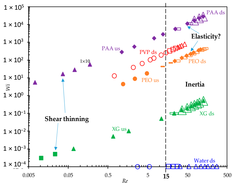
Figure 10. Summary of flow regimes in the Wi - Re space for the flow of Newtonian and non-Newtonian fluids through a contraction–expansion microchannel. Filled markers are for the upstream (us) flows at the contraction part and hollow markers are for the downstream (ds) flows at the expansion part of the microchannel: circles for no bending streamlines or vortices; squares for stable lip vortices; triangles for stable corner vortices; dashes for bending streamlines; diamonds for unstable or asymmetric corner vortices. The vertical dashed line indicates the Reynolds number, Re = 15 , at which the fluid inertia starts drawing apparent disturbances to the flow at the expansion of the microchannel. Note that the Weissenberg number has been assumed to be 0.01 and 0.1 for the pure water and XG solution, respectively, for the purpose of the graph.
