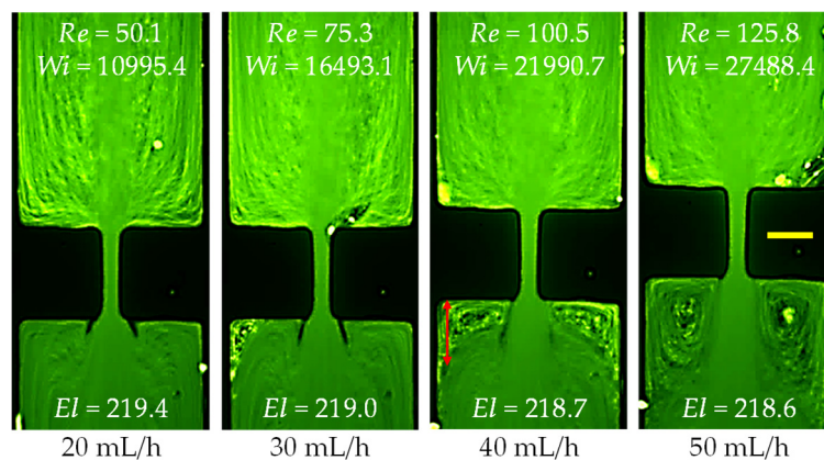
Figure 9. Strongly inertial flow (downward) of 200 ppm highly elastic and highly shear thinning PAA solution at the contraction–expansion region of the microchannel. The scale bar represents 100 \mu\text{m} .
