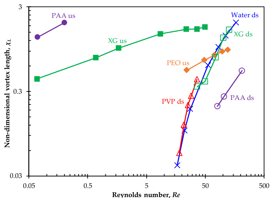
Figure 11. Non-dimensional vortex length, \chi_L = L_v/w , against the Reynolds number in the flow of Newtonian and non-Newtonian fluids through a contraction–expansion microchannel. Filled markers are for the upstream (us) vortices at the contraction part and hollow markers are for the downstream (ds) vortices at the expansion part of the microchannel. Note that only the size of stable vortex (either symmetric or asymmetric) is shown in the plot.
