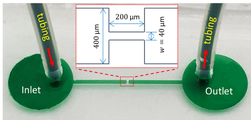
Figure 1. Picture of a fabricated 10:1:10 contraction–expansion microchannel with the inset displaying the dimensions.
