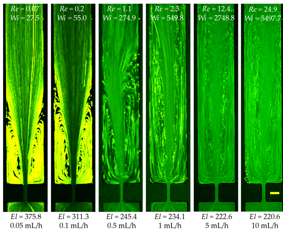
Figure 7. Inertialess ( Re < 0.1 ) or inertial flow (downward) of 200 ppm highly elastic and highly shear thinning PAA solution at the contraction–expansion region of the microchannel. The scale bar represents 100 \mu\text{m} .
