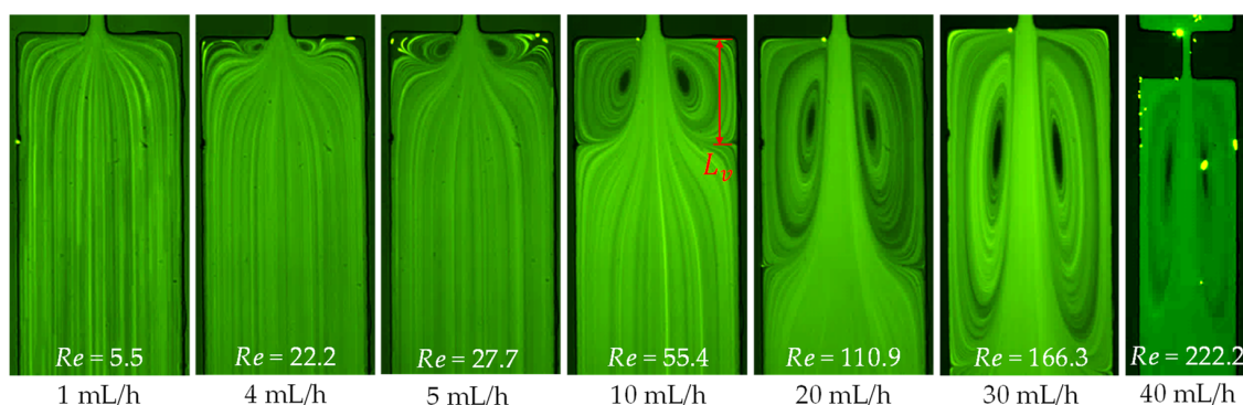
Figure 3. Inertial flow (downward) behavior of Newtonian water at the expansion part of the microchannel in a range of flow rates. No circulations are formed at the contraction part in any of the tested flow rates. The scale bars each represent 100 \mu\text{m} .
