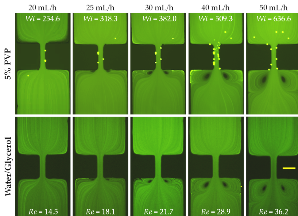
Figure 4. Comparison of the inertial flows (downward) of the viscosity-matched elastic polyvinylpyrrolidone (PVP, 5% in weight, top row) and Newtonian water/glycerol (40/60 in weight, bottom row) solutions at the contraction–expansion region of the microchannel. The scale bar represents 100 \mu\text{m} .
