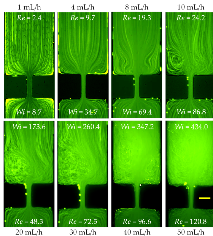
Figure 6. Inertial flow (downward) of 1000 ppm mildly elastic and weakly shear-thinning polyethylene oxide (PEO) solution at the contraction–expansion region of the microchannel. The scale bar represents 100 \mu\text{m} .
