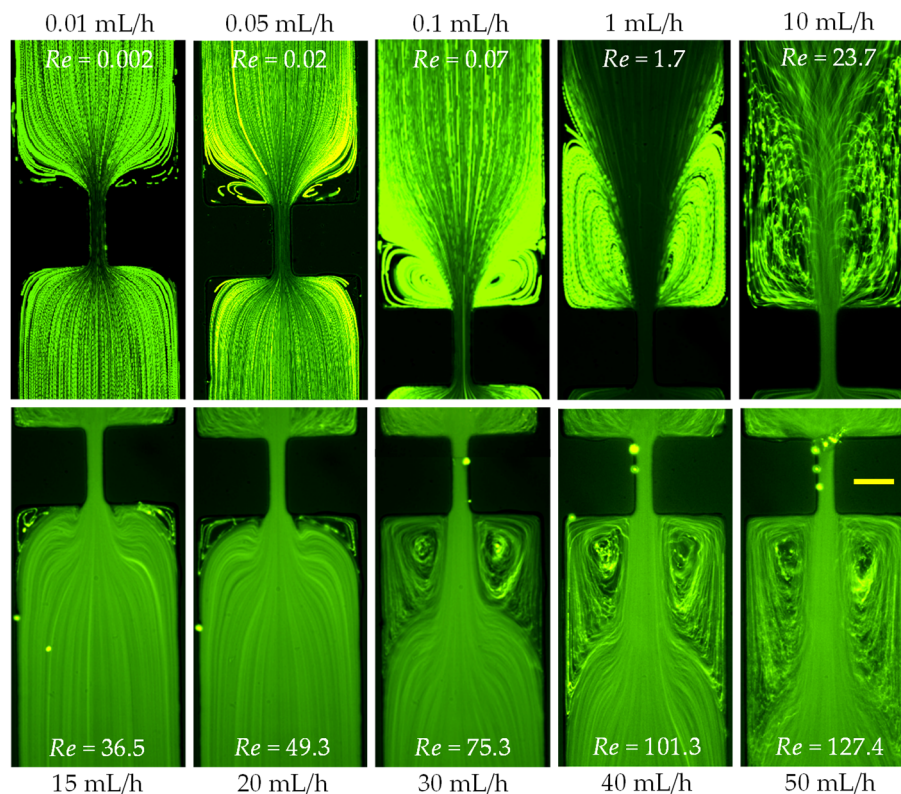
Figure 5. Inertialess ( Re < 0.1 ) or inertial flow (downward) of 2000 ppm shear-thinning XG solution at the contraction–expansion region of the microchannel. The scale bar represents 100 \mu\text{m} .
