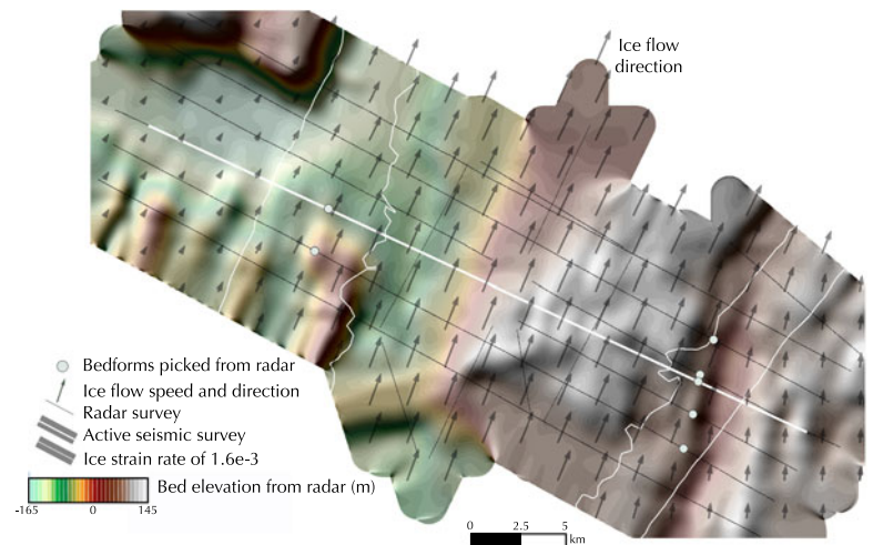
Fig. 5. Map of bed elevation showing picked bedforms (green dots), ice-flow direction (gray arrows, with size indicating flowspeed from 9 to 51 \text{m a}^{-1} ), seismic survey (white thick line), and radar survey (gray thin line). Areas bounded by the thin white line show where the ice-flow strain rate is greater than 1.6 \times 10^{-3} \text{ a}^{-1} . Site location corresponds to the inset in Figure 1a and covers the same region as Figure 1b.
