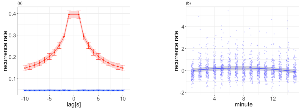
Figure 4: (a) Observed MdRQA recurrence rates at time lags 1-10s (red) versus randomly shuffled baselines (blue). Error bars indicate 95% confidence intervals. (b) Quadratic trend of time (minute) on regressing recurrence rate. Band around the fitted line denotes confidence interval, and blue points represent observations.
