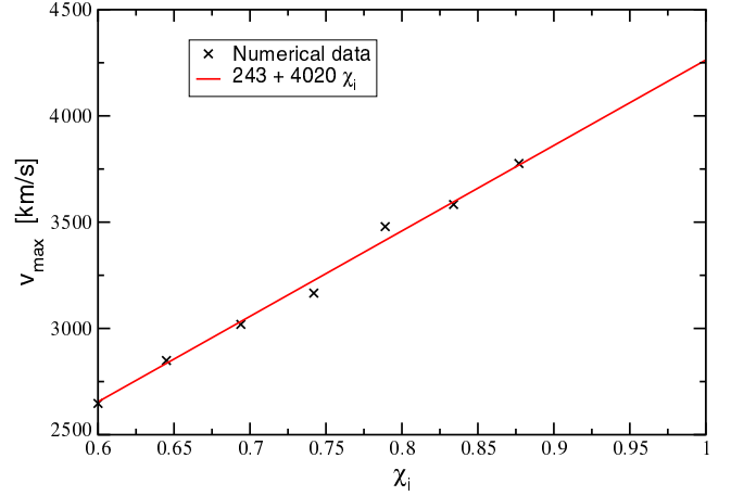
FIG. 4. The maximum recoil velocity v_{\max} for p/M = 0.075 as a function of the initial spin magnitude \chi_i . The curve represents the linear fit (4).
