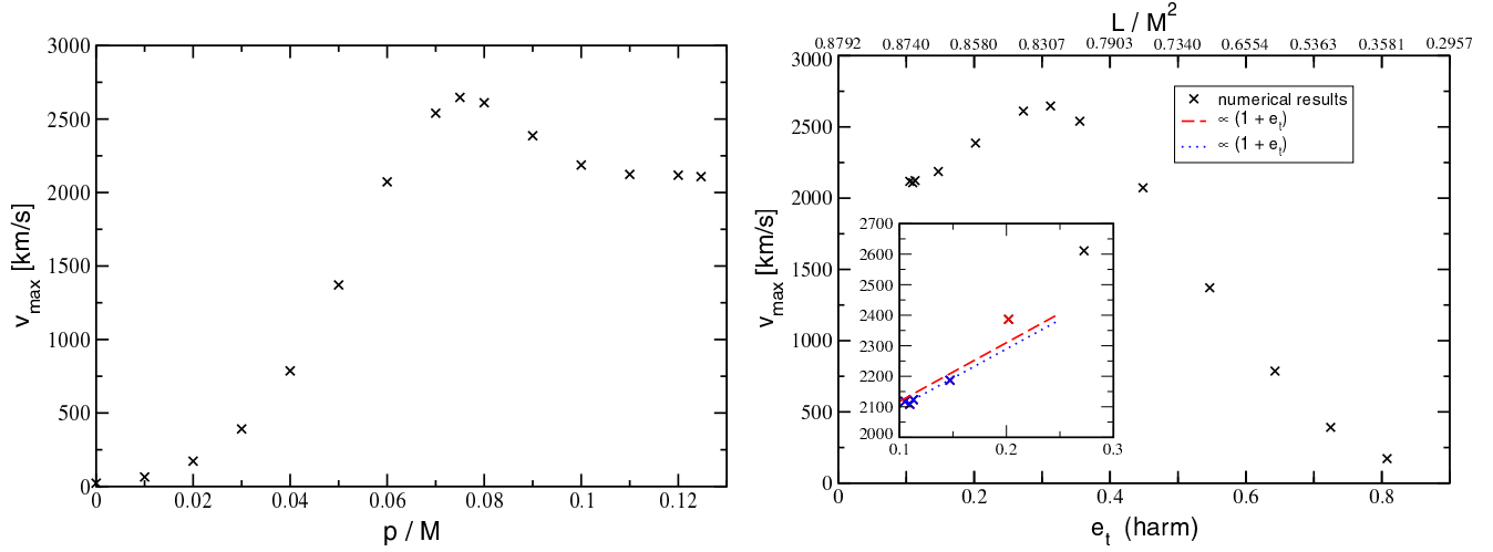
FIG. 1. Superkicks for eccentric binary BHs with equal masses and spins of magnitude \chi_1 = \chi_2 = 0.596 \approx 0.6 . Left : The maximum kick velocity v_{\text{max}} as a function of the linear momentum parameter. The largest kicks correspond to moderate eccentricity and exceed the quasicircular value by about 25%. Right : The maximum kick velocity v_{\text{max}} as a function of the eccentricity parameter e_t estimated in harmonic gauge. Labels on the upper horizontal axis display the corresponding initial orbital angular momentum L/M^2 of the binaries. The inset zooms in on the low-eccentricity regime and shows linear fits v_{\text{kick}} \propto (1 + e_t) obtained from the first four, blue data points (dotted curve), and also including the fifth, red data point (dashed curve). The increase of the recoil for small eccentricity is compatible with the (1 + e) scaling from close-limit calculations [44].
