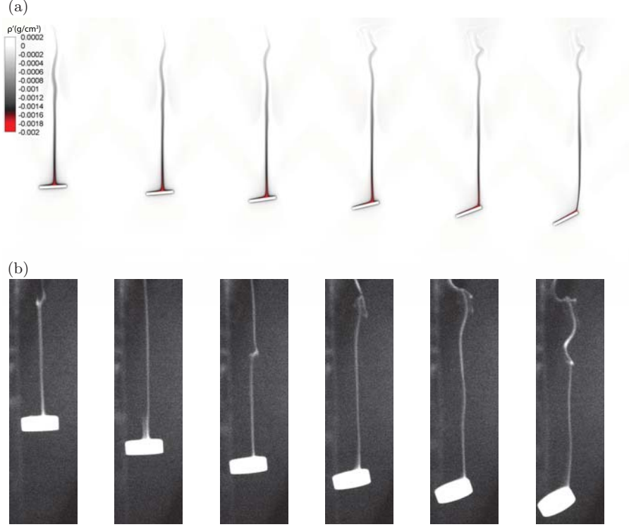
FIGURE 7. Examples of wake visualizations during phase 2 in experiments and numerics, the parameters chosen for each run are different. Maps of (a) density variations \rho^* = \rho - \rho_f for the numerical simulation (run N10), and (b) fluorescent dye for the experiment (run E14). At the first frame, Re \simeq 40 and Fr \simeq 0.75 for experiments and Re \simeq 17 and Fr \simeq 0.23 for numerics; each frame is separated by \Delta t = 2s , i.e. N\Delta t = 1 .
