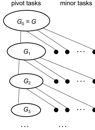
Fig. 2. Task Partitioning
