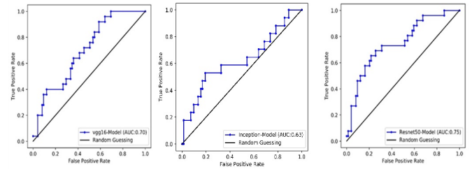
Fig. 7: Obtained ROC curve for different models.
