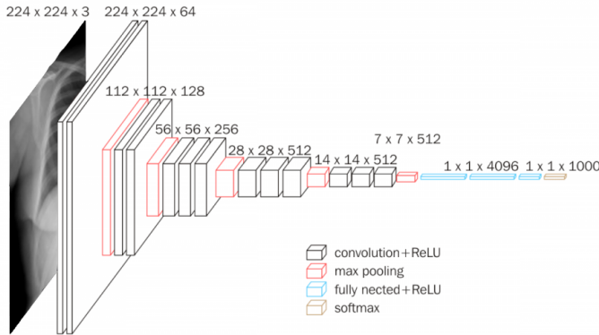
Fig. 5: The Proposed Architecture.
