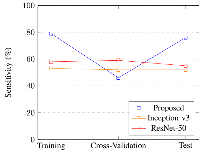
Fig. 11: Sensitivity of Datasets using three models: Proposed, Inception v3, and ResNet-50
