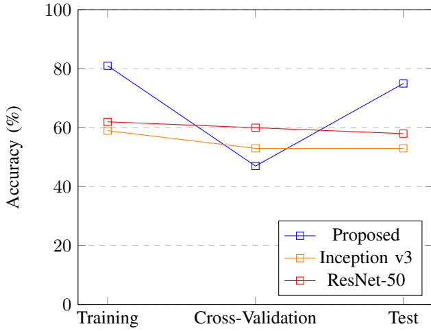
Fig. 8: Accuracy of Datasets using three models: Proposed, Inception v3, and ResNet-50
