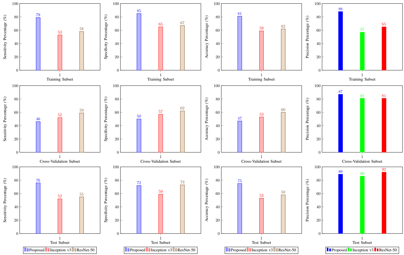
Fig. 12: Accuracy, Specificity, Precision, and Sensitivity of the three datasets: Training, Cross-Validation, and Test using Proposed, Inception v3, and ResNet-50 models
