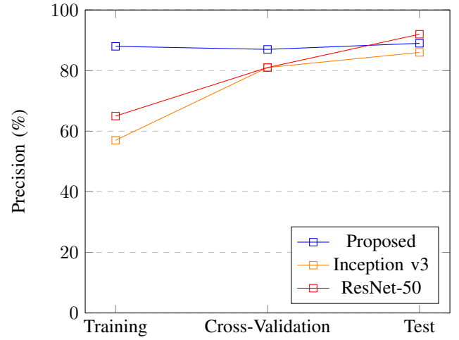
Fig. 10: Precision of Datasets using three models: Proposed, Inception v3, and ResNet-50
