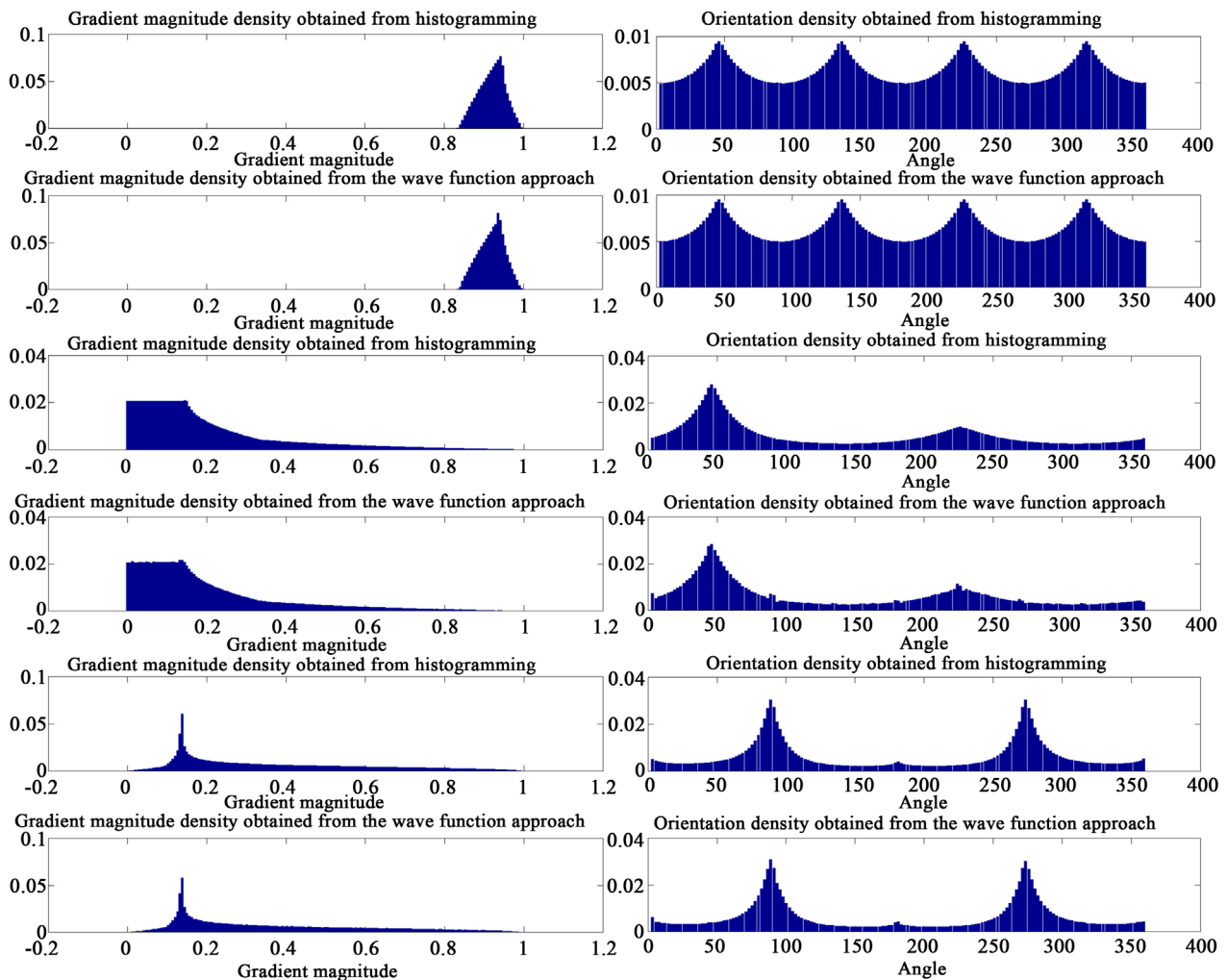
Figure 1. Comparison results. 1) Left: Gradient magnitude density, 2) Right: Gradient orientation density. In each sub-figure, we plot the density function obtained from histogramming and the wave function method at the top and bottom respectively.
