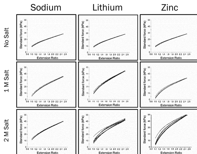
Fig. 5 Hysteresis testing of salt-loaded PAA samples. More significantly decreased recovery is evident in the 2 M LiCl and ZnCl 2 samples than in the NaCl samples.
