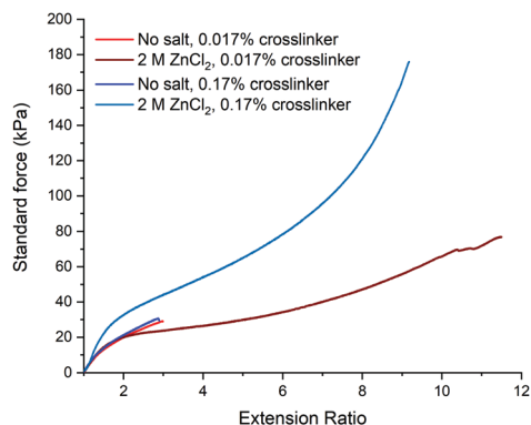
Fig. 6 Stress strain curves of PAA synthesized with 0.017% (reds) or 0.17% (blues) N,N' -methylenebisacrylamide either with no salt or 2 M \text{ZnCl}_2 .
