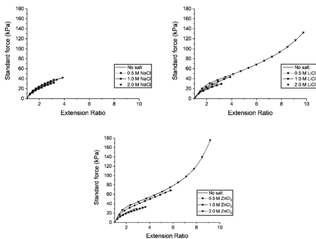
Fig. 4 Stress-strain curves of PAA loaded with sodium chloride (top left), lithium chloride (top right), and zinc chloride (bottom) at different salt loading levels of no salt (line), 0.5 M (circles), 1.0 M (squares) and 2.0 M (triangles).
