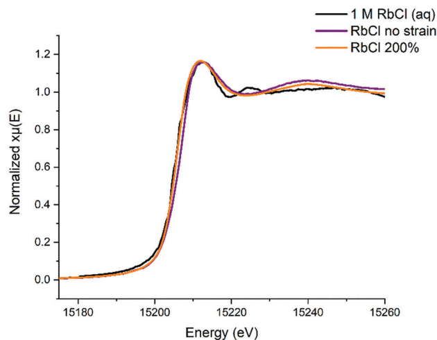
Fig. 10 XANES comparing aqueous RbCl, unstrained 2 M RbCl-PAA, and 2 M RbCl-PAA at 200% strain. The white line intensity across all samples is roughly similar.
