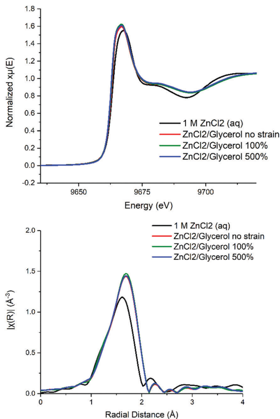
Fig. 8 (top) XANES of 2 M \text{ZnCl}_2 -loaded PAA in 50:50 water:glycerol showing little change in white line location and intensity. (bottom) EXAFS of the same samples showing a pronounced difference between the 1 M aqueous \text{ZnCl}_2 and the Zn-loaded samples.
