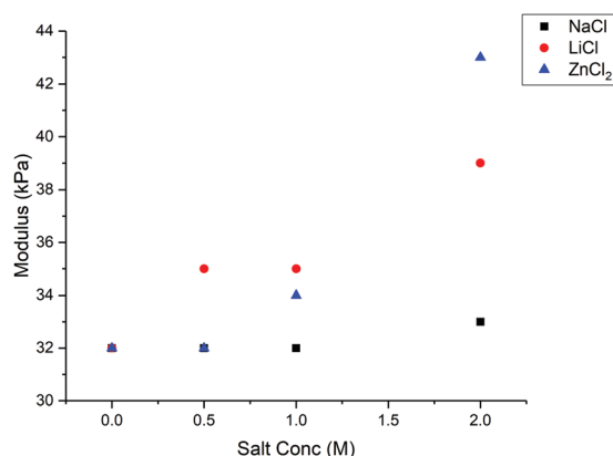
Fig. 3 Modulus vs. salt concentration for salt-loaded PAA samples. The highest modulus was exhibited by the 2 M ZnCl 2 samples, with samples with loading levels 1 M or lower maintaining similar moduli to those of samples synthesized without salt.
