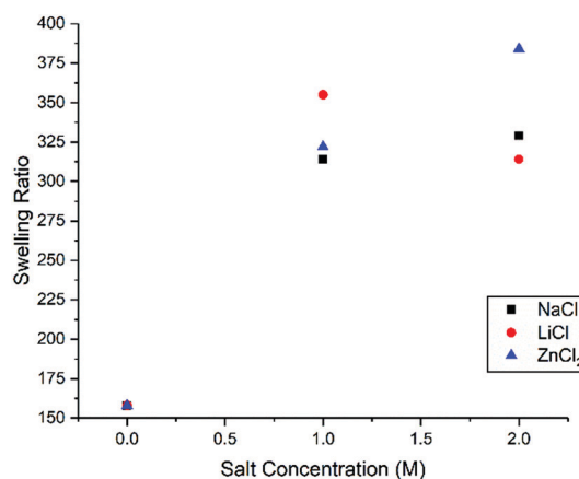
Fig. 2 Equilibrium swelling ratio vs. salt concentration. ZnCl 2 samples exhibited the greatest amount of swelling overall. In general, the 2 M samples exhibited significantly increased swelling as compared to the samples with no salt.
