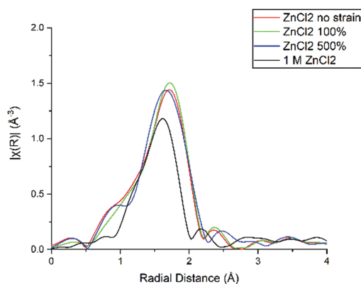
Fig. 9 EXAFS of 2 M \text{ZnCl}_2 -loaded PAA samples made with 6 M AAC rather than 3 M AAC. Once again, there is less apparent change upon strain as compared to the 3 M PAA samples discussed above.
