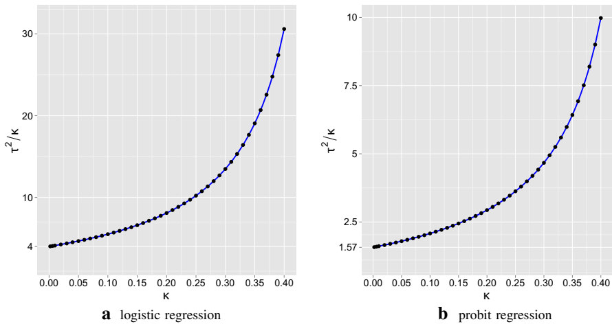
Fig. 3 Ratio of asymptotic variance and dimensionality factor \kappa as a function of \kappa
