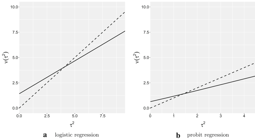
Fig. 7 The variance map for both the logistic and the probit models when \kappa = 0.3 : (solid line) variance map \mathcal{V}(\tau^2) as a function of \tau^2 ; (dotted line) diagonal
