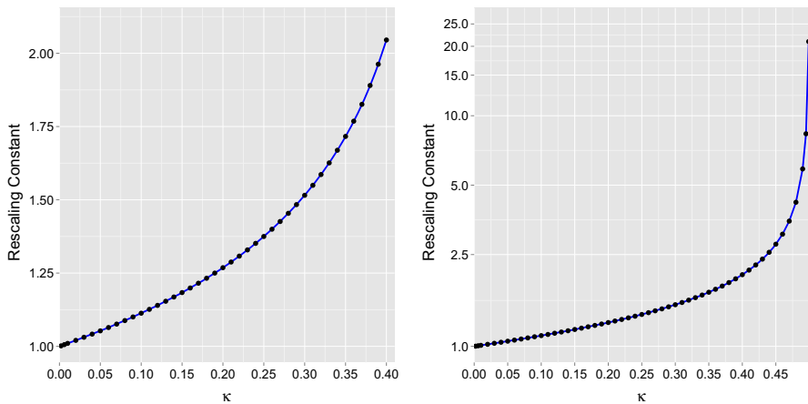
Fig. 2 Rescaling constant \alpha(\kappa) as a function of \kappa for the logistic model. Note the logarithmic scale in the right panel. The curves for the probit model are nearly identical
