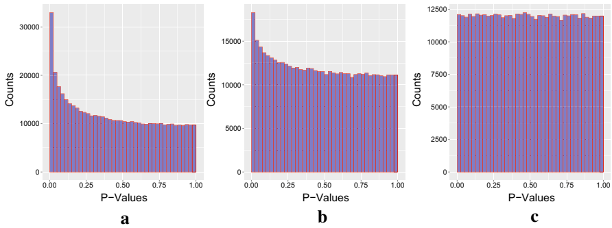
Fig. 4 Histogram of p -values for logistic regression under i.i.d. Bernoulli design (this is, therefore, not the setup of Fig. 1), when \beta = \mathbf{0} , n = 4000 , p = 1200 , and \kappa = 0.3 : a classically computed p -values; b Bartlett corrected p -values; c adjusted p -values
