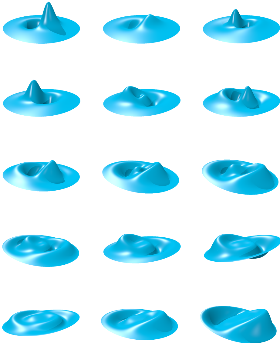
Figure 7: Evolution of the interface at t = 0, 1/80, 2/80, \dots, 14/80 . We use M = 4, J = 20, N = 40, K = 2, h = 0.5, \epsilon = 0.01 and RK4 for the time evolution with a time-step of \Delta t = 1/1200 .
