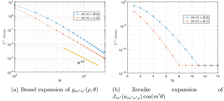
Figure 2: (a) L^\infty errors in the representation of the corrected Zernike polynomial g_{m'n'}(\rho, \theta) in terms of Bessel functions decay algebraically. Observe that the decay rate is N^{-5/2} which is in agreement with the expected N^{-(2p+1/2)} with p = 1 since only the first compatibility condition is satisfied by g_{m'n'} . (b), the L^\infty errors in the representation of J_{m'n'}(a_{m'n'}\rho)e^{im'\theta} in terms of Zernike polynomials decay exponentially.
