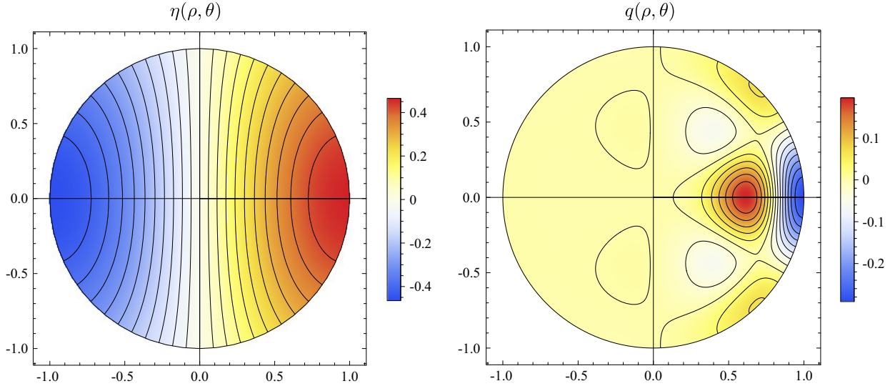
Figure 5: Contour plots of \eta(\rho, \theta) and q(\rho, \theta) corresponding to \epsilon = 0.8 in Figure 4. Here \eta(\rho, \theta) = 0.8J_1(a_{11}\rho)\cos\theta and q(\rho, \theta) is given by (6.4) with (m', n') = (3, 2) . The TFE recursion converges in spite of the large deviation of \eta(\rho, \theta) from the flat state.
