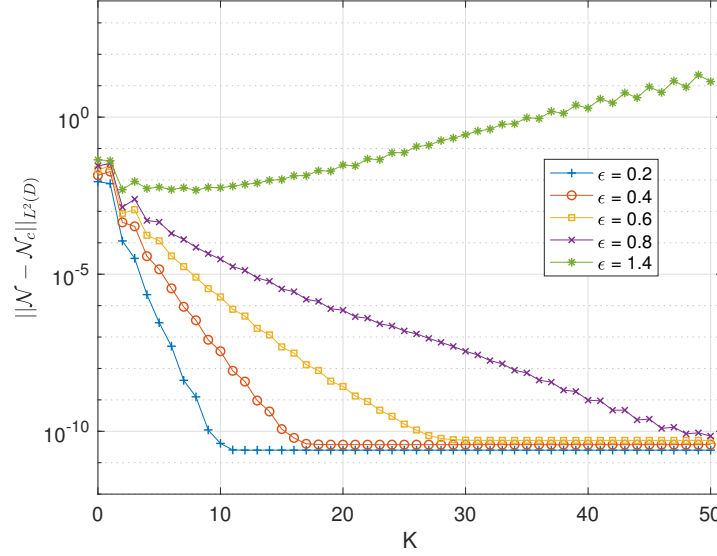
Figure 4: Errors in Neumann data vs. TFE order K for different values of \epsilon , for (m', n') = (3, 2) in Fig. 3. Observe that the error decay, while still exponential, slows down as \epsilon is increased. For too large a value, the method fails to converge at all.
