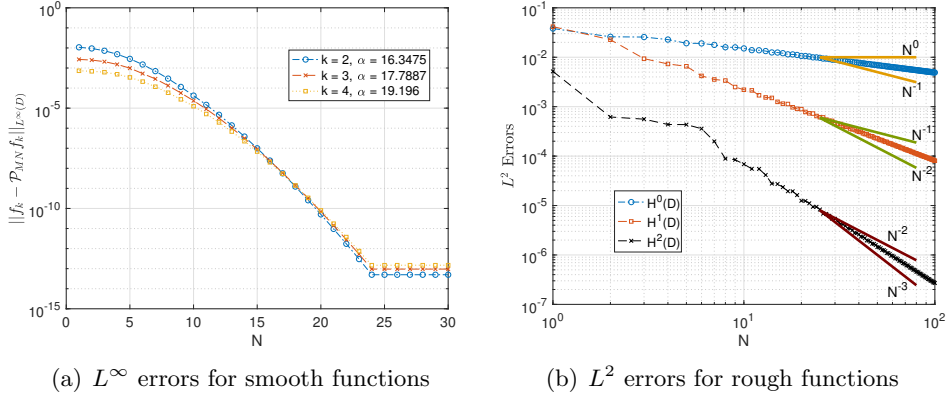
Figure 1: (a) L^\infty errors in the Zernike representation of f_k(\rho, \theta) = e^{-\alpha\rho^2} \rho^k \cos(k\theta) vs. N . Observe that the errors decay super-algebraically (in fact exponentially) in N , as established in Theorem 5.1, since f is infinitely differentiable, and that the same holds for pointwise errors. (b) L^2 error plots for Zernike representations of functions that belong to H^0(D) , H^1(D) and H^2(D) . The convergence is algebraic and controlled by N^{-s} for an H^s function.
