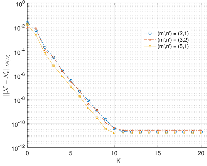
Figure 3: Convergence of Neumann data vs TFE order K for various Dirichlet conditions. The parameter choices are M = 32 , J = 20 , N = 42 , h = 1.0 and \epsilon = 0.2 .
