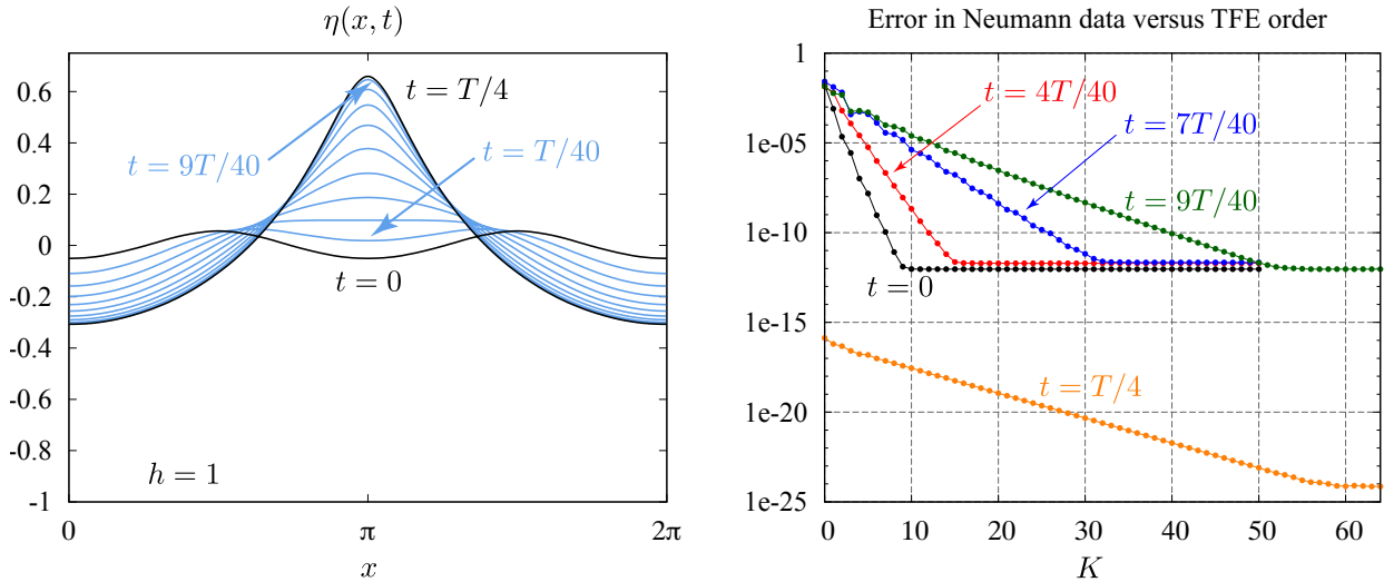
Figure 6: One-dimensional example showing that the transformed field expansion converges over the entire evolution of a large-amplitude standing water wave. (left) Evolution of solution B of Fig. 2 in [35], which has period T = 7.240 . Here we replaced the boundary integral method in [35] with the one-dimensional TFE code described in [34]. (right) The error in the computed Neumann data at each TFE order is measured against the boundary integral solution at the times shown.
