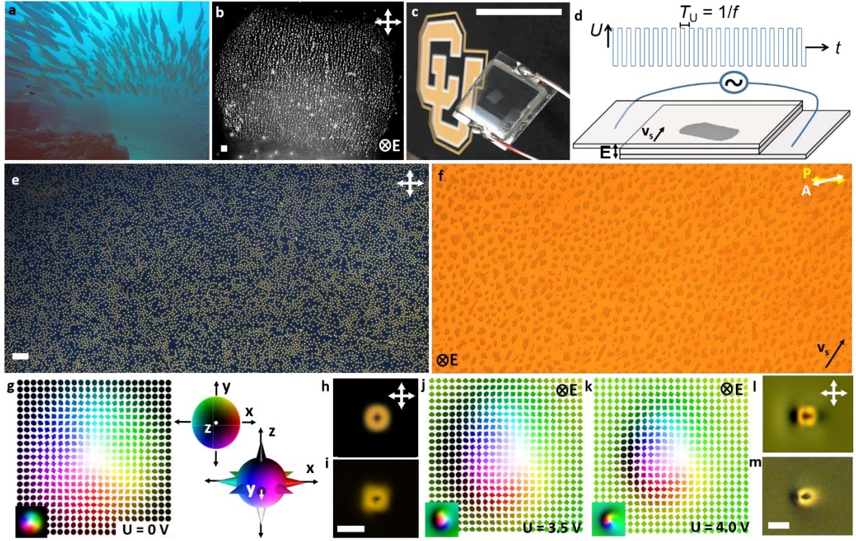
Figure 1 | Skymions and schooling. a , Underwater photograph of fish schooling. b , Zoomed-out grayscale polarizing optical micrograph of a school of skyrmions. The scale bar in the bottom left is 100 \mu\text{m} . c , Photograph of the skyrmion school shown in (b) , visible with the unaided eye as the cloudy region within the sample. The scale bar is 1 inch. d , Schematic of a sample with voltage application across the LC by using transparent electrodes on the inner surfaces of the confining substrates. The dark region within the schematic represents the moving skyrmion school shown in (b,c) . e, f , Low-magnification experimental polarizing micrographs of a region within the school at U=0\text{V} ( e ) and U=3.5\text{V} ( f ). The scale bar in the bottom left of (e) is 100 \mu\text{m} . g , Numerically-simulated \mathbf{n}(\mathbf{r}) of an individual skyrmion at U=0 shown by arrows colored according to points on the two-sphere \mathbb{S}^2 , as shown in the right-side inset. h,i , Computer-simulated polarizing micrograph ( h ) closely matches its experimental counterpart ( i ). Numerically-simulated \mathbf{n}(\mathbf{r}) of skyrmions at U=3.5\text{V} ( j ) and U=4.0\text{V} ( k ), with corresponding computer-simulated ( l ) and experimental ( m ) polarizing micrographs at U=4.0\text{V} . Bottom left insets in (g, j,k) are smoothly-colored representations of \mathbf{n}(\mathbf{r}) . The scale bars in (i) and (m) are 10 \mu\text{m} . Directions of \mathbf{E} , skyrmion motion velocity \mathbf{v}_s , U , T_U , double arrows denoting polarizer orientations and time t are marked throughout. Numerical simulations are based on material parameters of LC mixture of nematic MLC-6609 and right-handed chiral additive CB-15 (Methods) and d \approx p \approx 10 \mu\text{m} .
