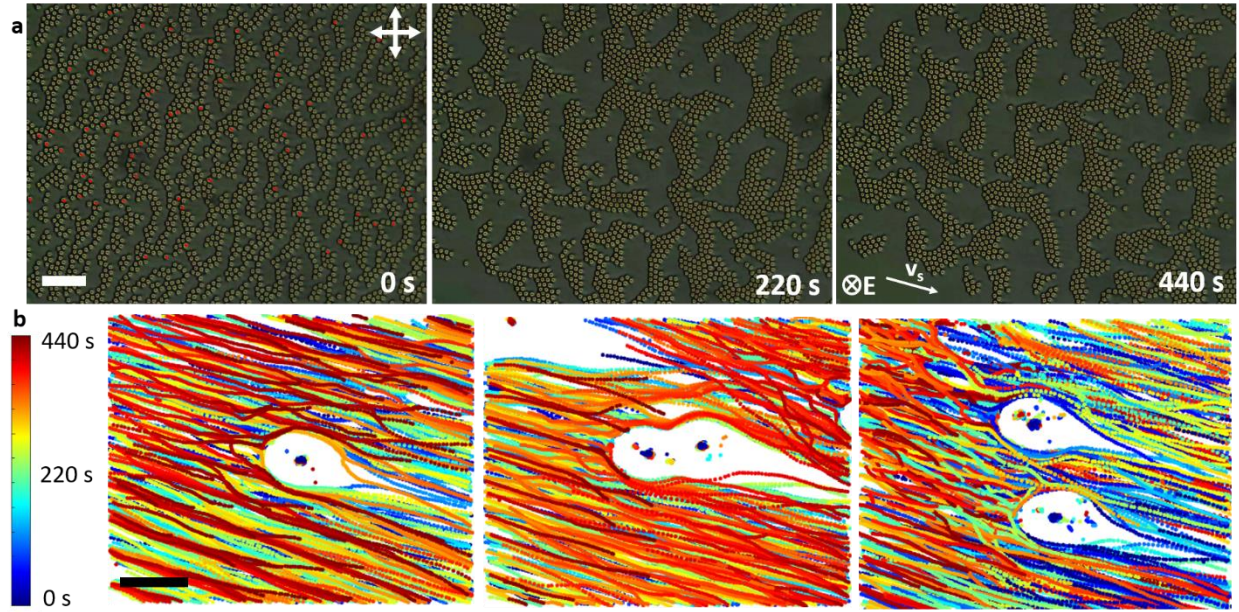
Figure 8 | Collective motion of skyrmion clusters within schools while bypassing obstacles. a, Polarizing micrographs of clustered skyrmion motion taken from the Supplementary Movie 1, where some skyrmions are pinned to the substrate and act as stationary obstacles (marked with red points in the first frame). The motion is powered by U=3 V at 60 Hz. Polarizer orientations are marked with white double arrows; direction of motion and electric field are marked on the last frame of (a). The elapsed time is shown in the bottom-right corners of micrographs. The scale bar is 100 \mu\text{m} . The chiral LC is the nematic host ZLI-2806 doped with CB-15. b, Examples of trajectories of skyrmion motion avoiding pinned obstacles, color-coded by the elapsed time according to the scheme shown on the left-side inset. Time-coded trajectories reveal details of skyrmions bypassing one obstacle (left), two connected obstacles (middle) and two separated obstacles (right). The scale bar is 50 \mu\text{m} .
