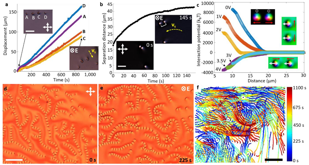
Figure 2 / Pair interactions and motions of individual and two-to-hundreds assemblies of skyrmions. a , Comparison of motions of individual and pairs of skyrmions labeled as in the video frames shown in insets. Applied voltage is U=4.5\text{V} , oscillated at f=2\text{Hz} ; high-frequency 1\text{ kHz} carrier signal is used (see Methods), indicating that these motions are not caused solely by the dynamics of ions 24 . The scale bar is 100\text{ }\mu\text{m} . b , Pair separation distance versus time during skyrmion motion along the arched trajectory, with insets showing skyrmions in the first and last frames and the pair separation distance labeled on the last frame. Motion was powered by U=4.5\text{ V} and at f=1\text{ Hz} oscillation frequency, with high carrier frequency of 1\text{ kHz} . Velocity directions \mathbf{v}_s are marked in insets of (a,b) with yellow dashed arrows. The scale bar is 50\text{ }\mu\text{m} . c , Pair interaction potential for skyrmions in motion at various voltages and at f=75\text{Hz} . Insets show smoothly-colored simulated \mathbf{n}(\mathbf{r}) configurations that follow the color scheme in Fig. 1g and reveal the presence of attractions or repulsions. Gray arrows mark the preimage vectors and red arrows represent attractive or repulsive forces between skyrmions. d , e , Frames from video showing temporal evolution of chains with hundreds of skyrmions at U=4.2\text{V} oscillated at f=2\text{ Hz} . f , Time-colored trajectories representing skyrmion motions over a time period of 1100\text{ s} , with the right-side inset showing the time-color scheme. The scale bars in (d) and (f) are 100\text{ }\mu\text{m} . The chiral LC is MLC-6609 doped with left-handed chiral additives (a,b) ZLI-811 and (d, e) QL-76. White double arrows denote crossed polarizers for all micrographs in this figure. E is marked in (e) and in the last frame of insets in (a,b) . The elapsed time is marked in the bottom-right of frames.
