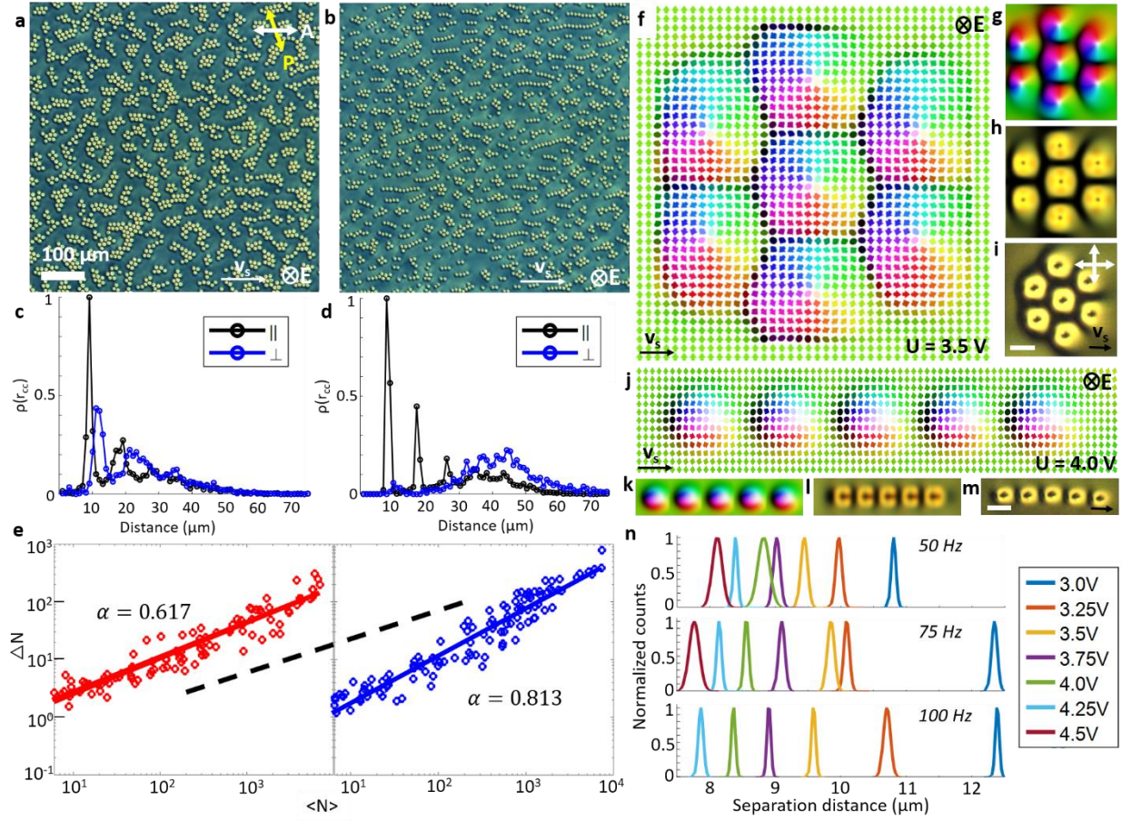
Figure 5 | Schools of skyrmions with internal clusters and chains. a,b , Polarizing micrographs show schooling of skyrmions with clusters at U=3.5\text{V} ( a ) and chains at U=4.0\text{V} ( b ), where f=50\text{Hz} . The scale bar in ( a ) is 100\text{ }\mu\text{m} . c,d , Normalized skyrmion count distributions \rho_{\perp}(r_{cc}) and \rho_{\parallel}(r_{cc}) for directions perpendicular and parallel to the motion directions for clusters ( c ) and chains ( d ) shown in ( a ) and ( b ), respectively. e , Log-log plots of \Delta N versus \langle N \rangle for clusters (red) and chains (blue); linear fits with slope \alpha values and a black dashed line with \alpha = 0.5 (for reference) are displayed. f,g , Computer-simulated moving cluster of seven quasi-hexagonally-assembled skyrmions at U=3.5\text{V} displayed using arrows colored according to the color scheme in Fig. 1g ( f ) and corresponding smoothly-colored representation of \mathbf{n}(\mathbf{r}) ( g ). h , Simulated and i , experimental polarizing optical micrographs of a similar moving cluster. j,k , Simulated moving linear chain of five skyrmions at U=4.0\text{V} ( j ) with corresponding smoothly-colored \mathbf{n}(\mathbf{r}) representation ( k ). l , Simulated and m , experimental polarizing micrographs of the moving chain. Scale bars in ( i ) and ( m ) are 10\text{ }\mu\text{m} . Upon turning voltage off and on again while minimizing \mathbf{n}(\mathbf{r}) , the clusters in ( f,j ) shift laterally within the computational volume by about \sim 0.5p . n , Experimental normalized distributions for inter-skyrmion distance in chains during motion versus U for f=50, 75 and 100\text{ Hz} . Polarizer orientations (double arrows), \mathbf{v}_s and \mathbf{E} are labeled throughout. The LC is the nematic ZLI-2806 doped with the chiral additive CB-15.
