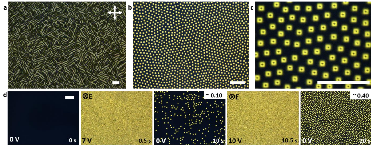
Figure 9 | Generation of skyrmions by relaxing electrohydrodynamic instabilities. a-c , Polarizing micrographs (at different magnifications) of a dense skyrmion array created by relaxing the electrohydrodynamic instability. The scale bars are 100 \mu\text{m} . d , Polarizing micrographs showing the as-prepared sample initially without skyrmions at no applied fields (left image), electrohydrodynamic instability at U=7\text{V} (2nd image from the left), skyrmions at low number density forming upon switching back to U=0 and relaxing the sample from electrohydrodynamic instability (3rd image from the left), electrohydrodynamic instability in the same sample area upon again applying U=10\text{V} (4th image from the left), and, finally, skyrmions at high number density forming upon switching back to U=0 again and allowing the instability to relax (5th image from the left). These images illustrate the control of the initial skyrmion packing fraction (by area, displayed in the top-right of the images), where the amplitude of U used to generate electrohydrodynamic instabilities correlates with the ensuing skyrmion number densities. White double arrows denote crossed polarizer orientations. Elapsed time, skyrmion packing fraction by area, applied voltage, and direction of \mathbf{E} are marked in the corners of micrographs. The used electric field frequency was 10Hz.
