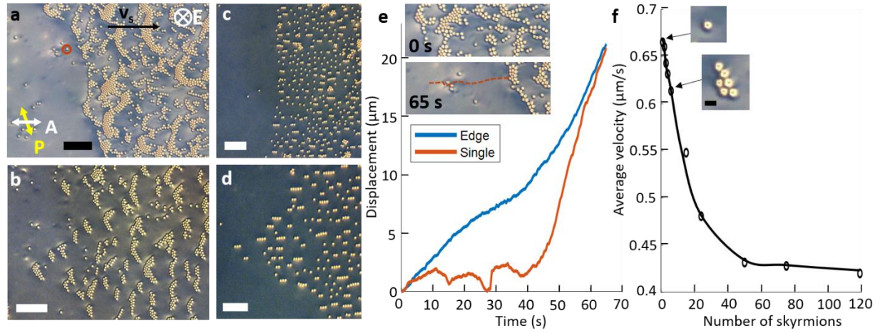
Figure 6 | Edges of dynamic skyrmion schools. a , Polarizing micrograph, extracted as a still frame from Supplementary Movie 6, displaying the edge of a school of skyrmions. b-d , Polarizing micrographs displaying different well-defined school boundaries. The scale bars in (a-d) are 100\ \mu\text{m} . e , Displacement of a single skyrmion compared to the school's edge, derived from frames of the Supplementary Movie 6, with insets showing the moving edge with time. The trajectory of a single skyrmion (highlighted with an orange circle) in (a) as it catches up to the edge is shown in the lower inset with an orange dotted line. f , Velocity of the skyrmion clusters versus the number of constituent skyrmions within the schools. The directions of v_s , uncrossed polarizer and analyzer (double arrows) and E are the same throughout as marked in (a) . The motion takes place at f=50\text{Hz} and (a, c) U=3.5\text{V} and (b, d) U=4.0\text{V} . The chiral LC mixture is ZLI-2806 doped with CB-15 (Table 1).
