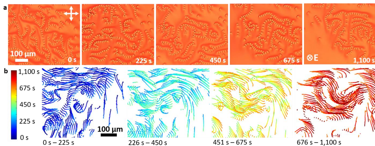
Supplementary Figure 2 | Details of the chain-like swirling motion of skyrmions. a , Temporal evolution of skyrmion chains at packing fraction \sim 0.005 and U=4.2\text{V} oscillated at f=2\text{ Hz} . b , Time-colored trajectories representing skyrmion motions between the frames displayed in (a) , with the left-side inset showing the time-color scheme for corresponding time periods marked beneath the plots. White double arrows denote crossed polarizers for all micrographs in this figure. The direction of E marked in the last frame of (a) corresponds to all figure parts. The elapsed time is marked on the frames. The scale bars are 100\text{ }\mu\text{m} . The chiral LC is MLC-6609 doped with QL-76.
