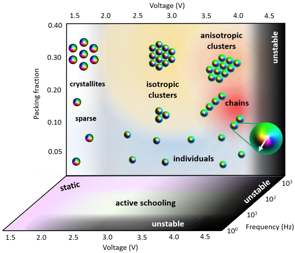
Figure 7 / Diagram of static and dynamic skyrmion assemblies and schools. A diagram of experimentally self-assembled dynamic and static structures versus packing fraction, f and U . The configurations shown are consistent across all f at which skyrmions are stable and shown as a single vertical panel for simplicity. Schematics of skyrmion assemblies in the insets are colored according to the scheme in the inset of Fig. 1g, with the enlarged inset displaying the preimage vector of a skyrmion at U=4.0 V.
