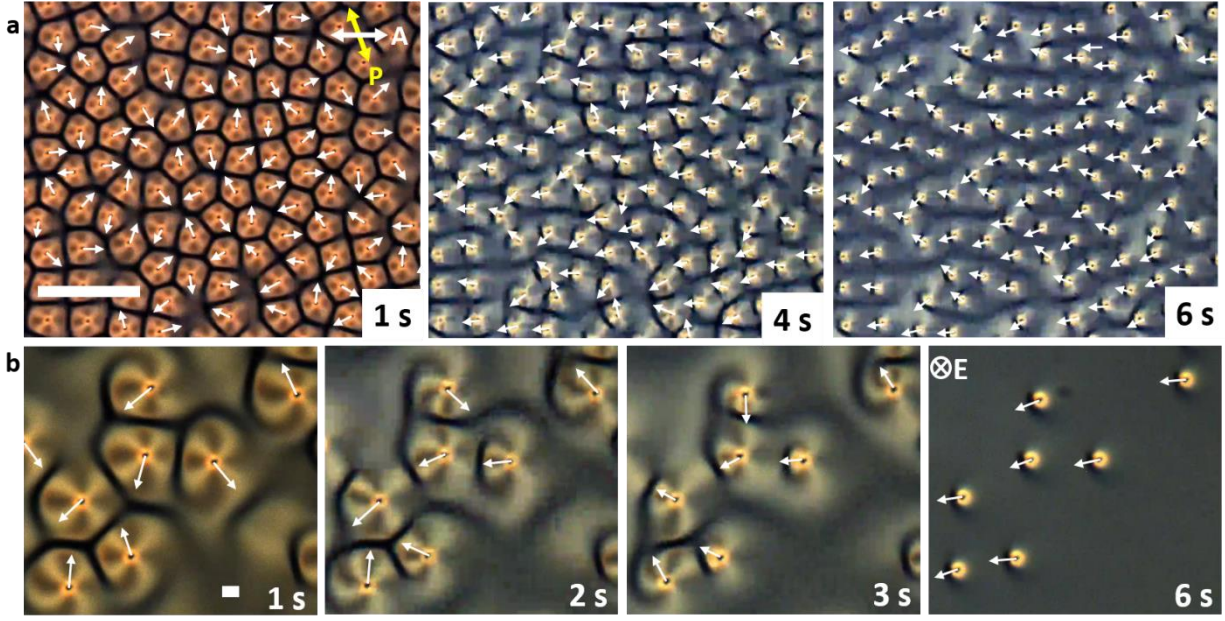
Figure 3 | Temporal evolution of skyrmion velocity vector orientations. This analysis is done at the onset of the ordering transition corresponding to Fig. 4d of the main text. a,b , Polarizing micrographs of (a) a higher number density region and (b) a lower number density region within the same sample at elapsed times marked on the images. White arrows point along the directions of skyrmion motion, representing the velocity unit vectors, \mathbf{v}_i . The applied voltage is U=3.5 V. The scale bars are (a) 100\ \mu\text{m} and (b) 10\ \mu\text{m} . Double arrows denote uncrossed polarizer and analyzer orientations and direction of voltage application in marked in the last frame of (b) . The chiral LC is the nematic host ZLI-2806 doped with CB-15.
