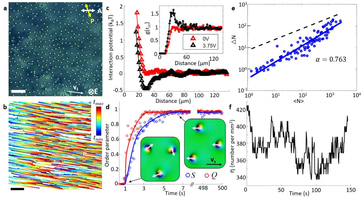
Figure 4 | Coherent skyrmion motion in a school. a , Experimental polarizing micrograph of moving skyrmions in a school without clustering for initial packing fraction of 0.09 by area at U=3.75 V and f=50 Hz. Polarizer and analyzer orientations are marked with double arrows and directions of \mathbf{E} and skyrmion motion are marked in the bottom-right corner. b , Trajectories of skyrmion motions color-coded with time according to the scheme shown in the right-side inset (where t_{\min}=0 and t_{\max}=72 s); these trajectories correspond to Supplementary Movie 5. The scale bars in (a) and (b) are 100 \mu m . c , Interaction potential (extracted from the radial distribution function g(r_{cc}) shown in the inset) of center-to-center distances r_{cc} for schooling skyrmions at conditions like in part (a) . d , Evolution of S and Q with time. Insets schematically show corresponding configurations colored according to the scheme in the inset of Fig.1g. e , Giant number fluctuation analysis using a log-log plot of \Delta N versus \langle N \rangle ; black dashed line indicates a slope of 0.5 for reference. f , An example of number density fluctuation during motion for a 400 \mu m \times 400 \mu m sample area. Such schools of individually dispersed, collectively moving skyrmions are observed at U=2.5-4.25 V and initial packing fractions within 0.01-0.09 by area. The LC is ZLI-2806 doped with right-handed additive CB-15 (Methods).
