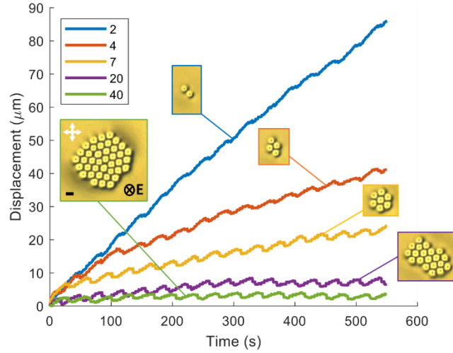
Supplementary Figure 1 | Skymion displacement versus time for different clusters. Displacement analysis of skymion clusters versus time at U=3.75 V at 2Hz oscillation frequency and at carrier frequency of 1kHz. The legend indicates the number of skymions in each cluster. Crossed polarizer orientations for all insets are marked with double arrows and the direction of \mathbf{E} is shown. The scale bar is 10 μm. The LC is MLC-6609 doped with ZLI-811.
