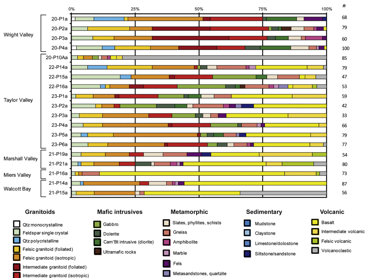
Fig. 4. Relative distribution of lithologies in 4–2-mm fraction petrographic analysis. n: total number of analyzed clasts.
