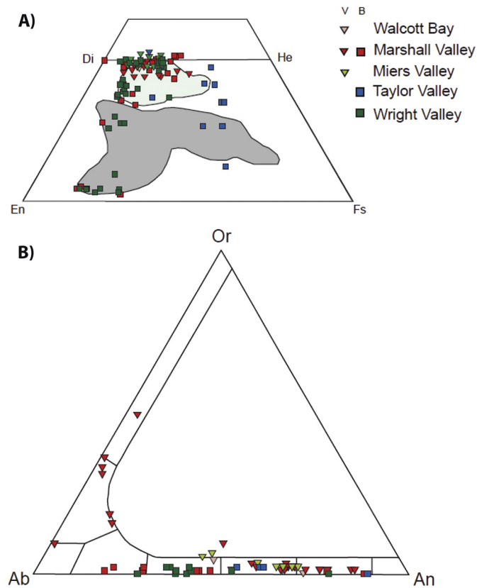
Fig. 7. (A) Pyroxenes diagram of analyzed clasts from Ross Sea Drift. Coloured fields show pyroxenes chemical composition of the Erebus Volcanic Province (after Gamble et al., 1986, light blue) and from the Ferrar Province (after Haban and Elliot, 1985, grey). (B) Feldspar ternary diagram of analyzed clasts. Abbreviations: V = volcanic lithic fragments; B = metamorphic and intrusive lithic fragments.
