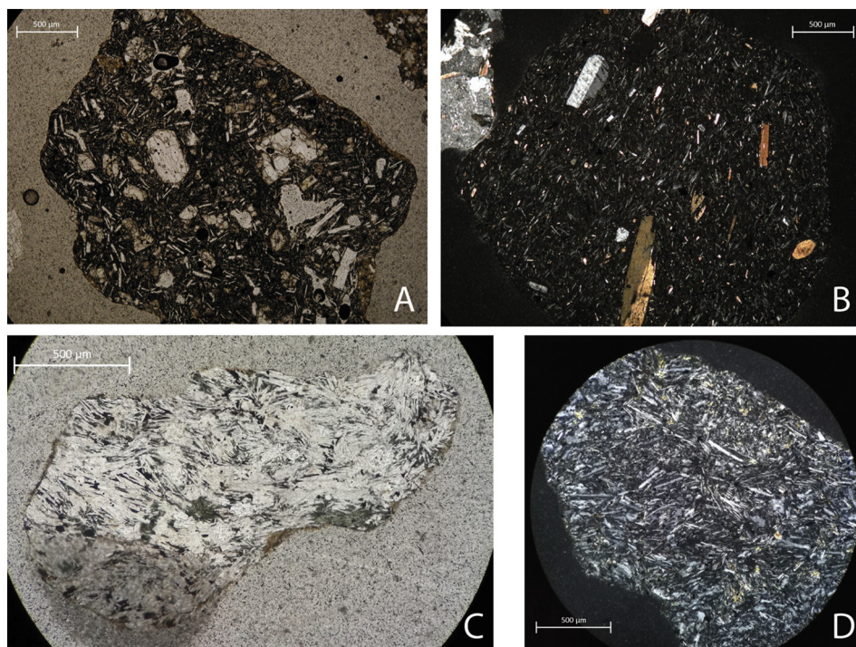
Fig. 6. Representative photomicrographs of volcanic clasts recovered in Ross Sea Drift samples. (A) microporphyritic clinopyroxene-olivine ipocrystalline basaltic clasts (plane polarized light, PPL, Walcott Bay sample); (B) microporphyritic sanidine-plagioclase-brown amphibole intermediate clast (crossed polarized light, XPL, Marshall Valley sample) (C) olocrystalline trachytic feldspars-green clinopyroxenes felsic clast (PPL, Marshall Valley sample); (D) same lithology as C (XPL, Marshall Valley sample).
