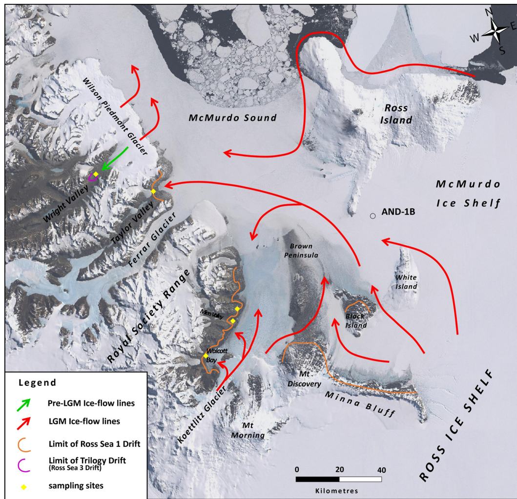
Fig. 9. Ice-flow reconstruction in McMurdo Sound during the LGM, based on the results of Wilson (2000), Anderson et al. (2017) and petrographic data from this study. Yellow points are location of sampling sites. Orange lines show the limit of Ross Sea 1 Drift (Denton and Marchant, 2000; Cox et al., 2012), while purple line marks the limit of Trilogy Drift in Wright Valley (Hall and Denton, 2005). Location of AND-1B is shown.
