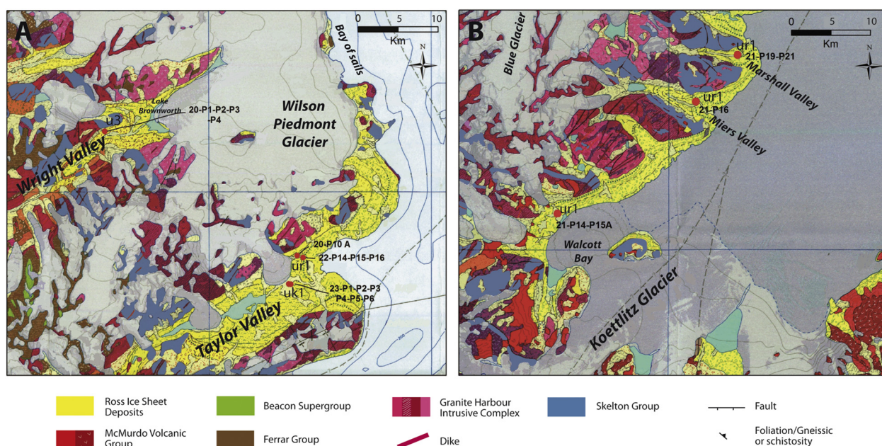
Fig. 2. Geological map of the areas from the two boxes (A and B) shown in Fig. 1, with sampling sites location and simplified legend. Maps from Cox et al. (2012). Deposits from which samples were taken are also shown, following the nomenclature given by Cox et al. (2012).
