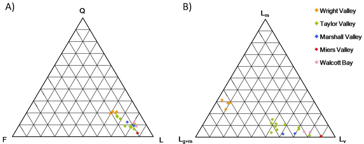
Fig. 5. (A) QFL diagram and (B) L_m - L_{g+m} - L_v diagram for 2 mm–425 \mu m point counting petrographic analysis. L_m = mafic intrusive lithic fragments; L_{g+m} = granitoids and metamorphic lithic fragments; L_v = volcanic lithic fragments. Data are normalized to 100.
