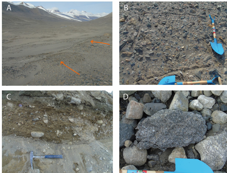
Fig. 3. (A) Lateral moraines of the Trilogy Drift on the north wall of the lower Wright Valley (arrows). (B) Detail of the sampled surface with scattered clasts of different lithologies. (C) Diamicton facies of Ross Sea 1 Drift from Marshall Valley incised stream, underlain by bedrock. (D) Cobbles of granitoids and plagioclase-phyric intermediate volcanites from the same site. Hammer is about 30 cm long, while shovel is 1 m long.
