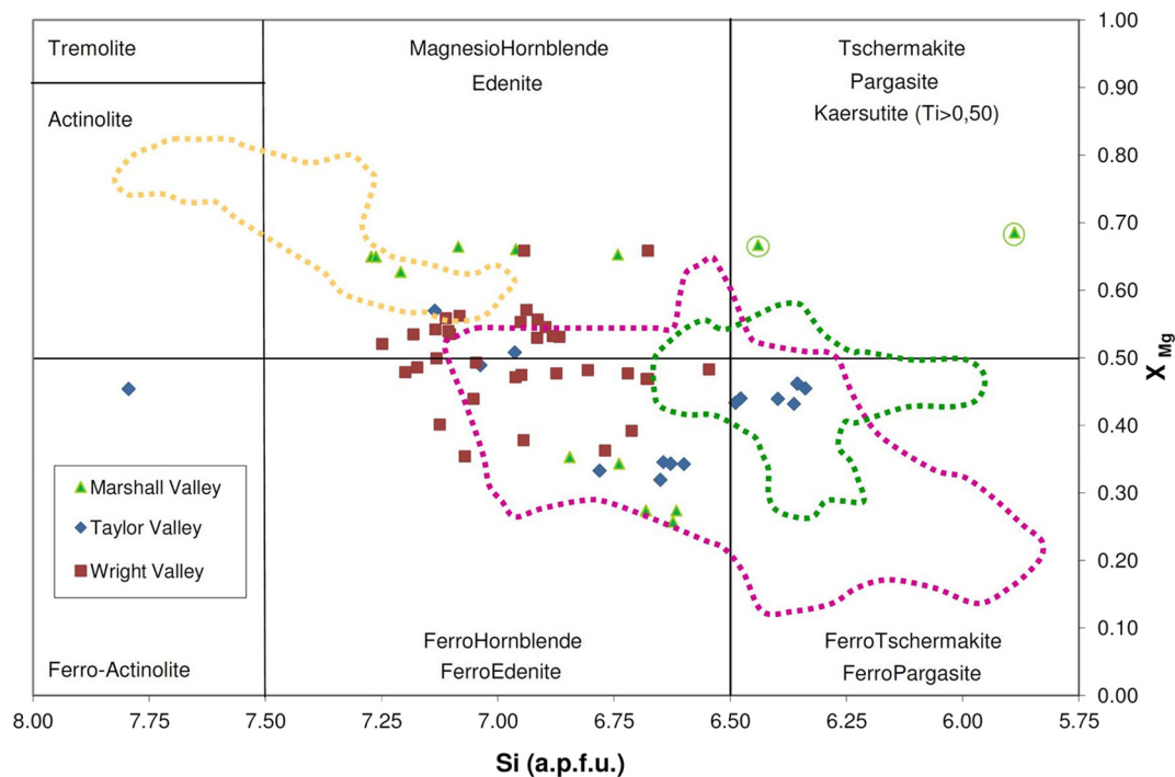
Fig. 8. Calcic-amphiboles classification (Leake et al., 1997) for Ross Sea Drift clasts. Coloured fields are amphibole compositions from known bedrock sources (Talarico et al., 2011, 2013): yellow = Skelton-Mulock glacier area; purple = Southern Victoria Land granitoids; green: Britannia Range area. Circled spots are kaersutite amphiboles ((Na + K) A ≥ 0.50 and Ti > 0.50 a.p.f.u.).
