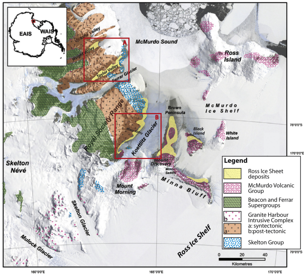
Fig. 1. Simplified geologic map of the southern Victoria Land in Antarctica. The red boxes refer to the sampling areas (the same are enlarged in Fig. 3 ). (A): Wright and Taylor valleys; (B): foothills of the Royal Society Range (RSR). Geologic map is taken from Sandroni and Talarico (2011) and Cox et al. (2012) .
