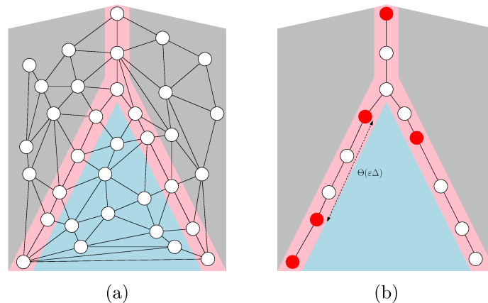
Figure 1: (a): Separator paths that divide a planar graph H into two components (corresponding to two children of the root of the decomposition tree \mathcal{T} ). (b): Portals along the separator.
