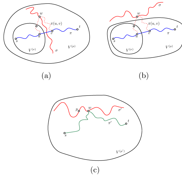
Figure 2: Detour through a vertex of a separator path \sigma in Claim 1, where \sigma may be internal, as in (a), or external, as in (b). Detour through a portal in Claim 2 in (c).
