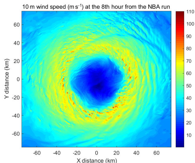
Figure 3. Instantaneous 10 m surface wind speeds of Hurricane Isabel (2003) at the 8th simulation hour by a WRF LES that uses the 3-D NBA SGS model.
