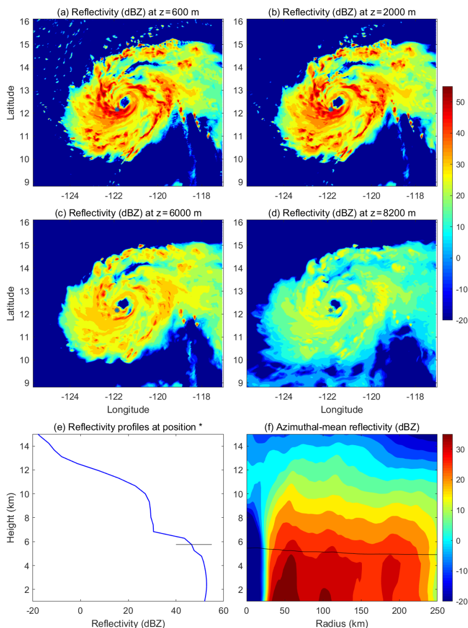
Figure 5. (a)–(d) HWRP-simulated radar reflectivity of Hurricane Jimena (2015) at different altitudes ( z = 0.6, 2.0, 6.0 , and 8.2 km) at 12:00 UTC, 28 August 2015. (e) Vertical profile of radar reflectivity at a location in the eyewall marked by an asterisk in (a)–(d). (f) Azimuthal-mean radius–height structure of radar reflectivity. Black line in (e) and (f) indicates the freezing line.
