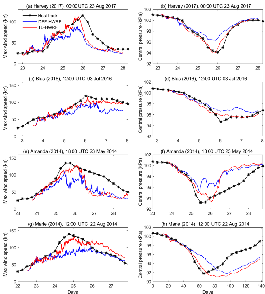
Figure 13. HWRP-simulated maximum wind speed and storm central pressure of four other major hurricanes, Harvey (2017), Blas (2016), Amanda (2014), and Marie (2014), compared with the best-track data (black curves). Blue curves: DEF-HWRF. Red curves: TL-HWRF.
