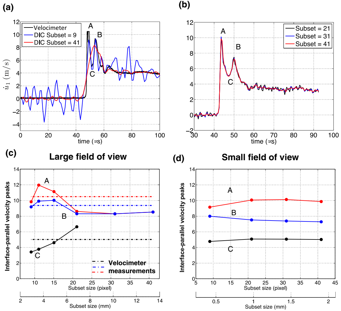
Fig. 14 (a-b) Velocity time histories for a pixel just below the interface and at the center of the field of view for the large and small fields of views, respectively. A velocimeter measurement corresponding to the same location is included for comparison, for the case of the large field of view. (c-d) Interface-parallel velocity vs. subset size for the case of large and small fields of view, respectively. The two peaks (denoted A and B in Fig. 14(a) and (b)) and the troughs (denoted as C) in the velocity time history are tracked as a function of the subset size. Solid datapoints indicate the DIC measurements. Velocimeter measurements (available only for the large FOV) are reported as dashed lines
