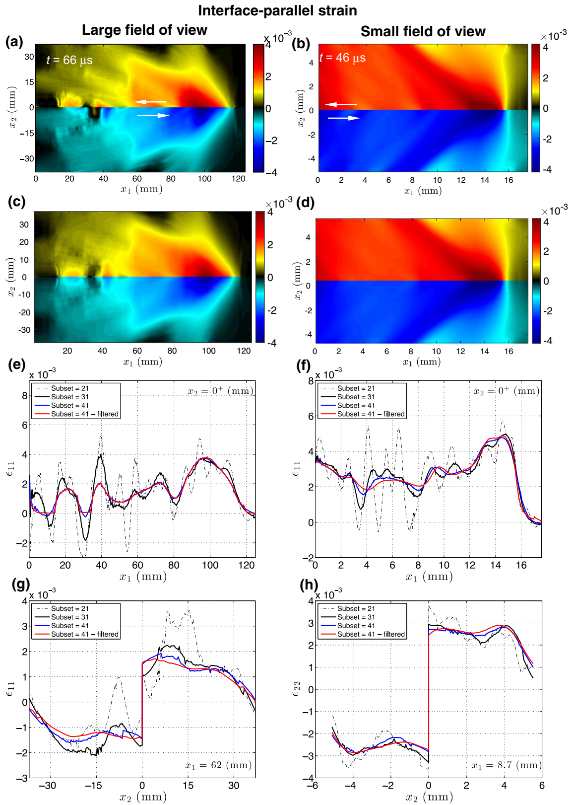
Fig. 11 Interface-parallel strain for the large (left column) and small (right column) fields of view. Full-field strain maps obtained (a-b) by using a subset size of 41 \times 41 \text{ pixels}^2 and filtering the displacement fields, and (c-d) by also including the symmetry adjustment. (e-f). Interface-parallel strain vs. position along the interface. (g-h) Interface-parallel strain vs. position perpendicular to the interface
