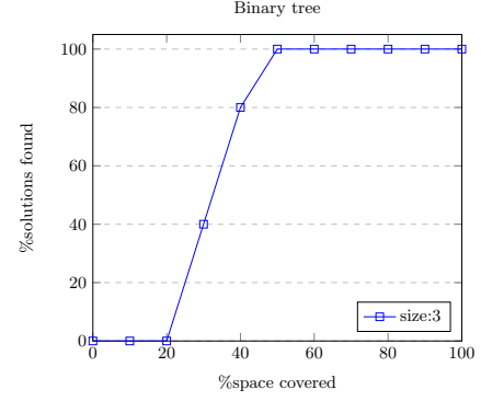
Figure 3: Korat solving of the binary tree constraints.
