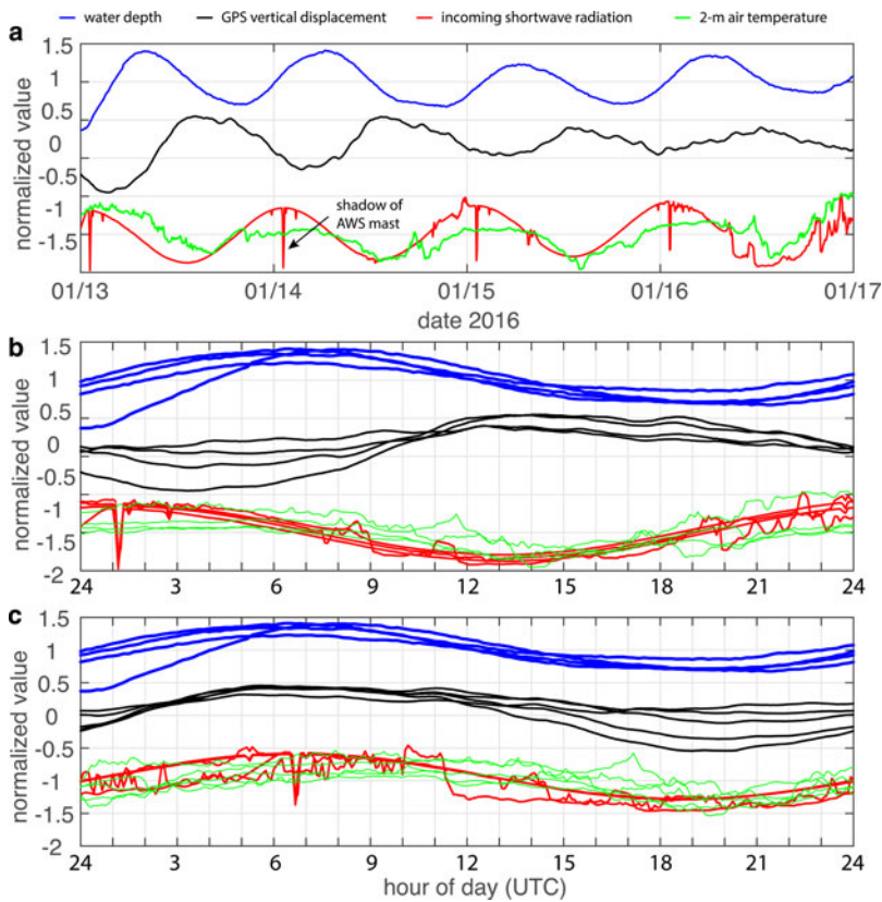
Fig. 4. (a) Normalized observed variables: water depth \eta , ice-shelf elevation ( \zeta + T ), incoming shortwave radiation, and 2-m air temperature over the 4-d period (13–17 January 2016) when water-depth fluctuations were most pronounced and where insolation was principally clear sky (Fig. 3). A legend signifying pairing of variables and line colors is provided above panel (a). Downward spikes in incoming shortwave radiation are caused by the AWS mast shadowing the radiometer. Normalization is accomplished by dividing the observed signal by the difference between maximum and minimum values over the 4-d period. Ice-shelf elevation was smoothed by a 1 h running mean of the GPS data. The water-depth time series has additionally had its mean and linear trend removed. (b) Each day's variation is plotted as a function of that day's time-of-day (UTC) to assess consistency of timing relationships and to judge time lags. (c) The normalized series of ice-shelf elevation must be shifted forward in time by 16.5 h, and the normalized shortwave input by 5.5 h, respectively, to align peak-to-peak with the meltwater-depth observation.
