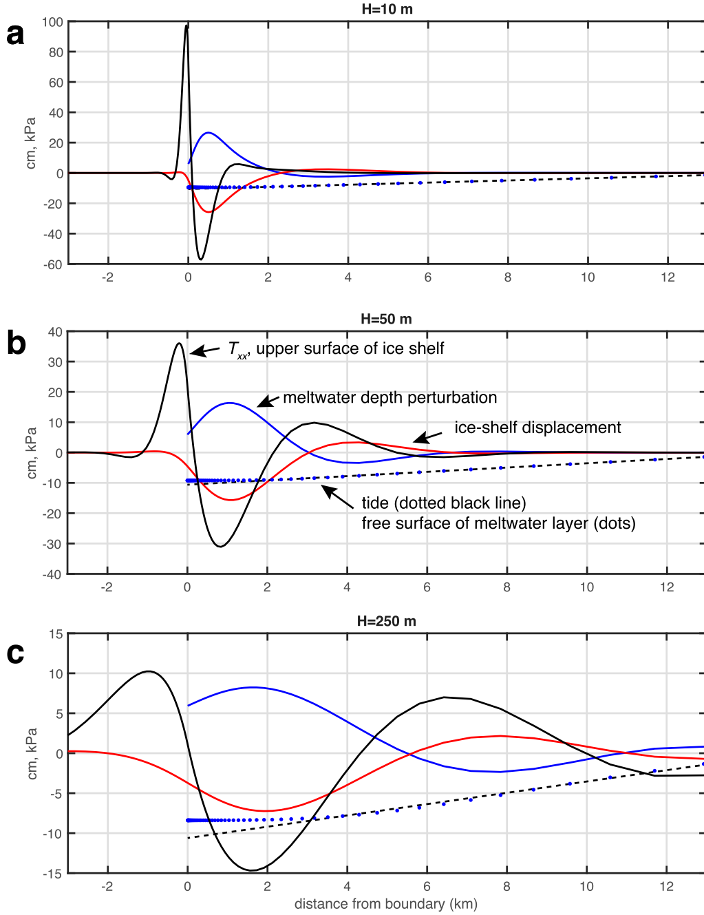
Fig. 10. Meltwater-layer depth perturbation ( \eta , cm, blue line), ice-shelf deflection due to purely elastic flexure ( \zeta , cm, red line), tide ( T , cm, dashed black line), free-surface of meltwater layer (blue dots) and ice-shelf stress at the upper surface ( T_{xx} , kPa, black line) for three representative ice thicknesses ( H = 10, 50 and 250 m, panels (a–c), respectively). The time for which the solution is shown is \pi/4 units of phase after low tide (when the slope of T is maximum), and is chosen to show the depth of the meltwater-layer perturbation at its largest. Note the change in scale for each panel.
