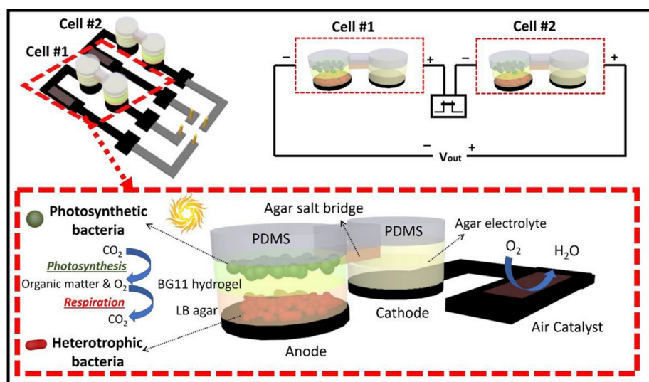
Fig. 1. A conceptual schematic diagram of the bio-solar power system. Each cell has a dual-chambered configuration with solid-state anolyte, catholyte and salt bridge. Two cells are integrated in a well-designed microsystem and will be connected in series for powering an application.
