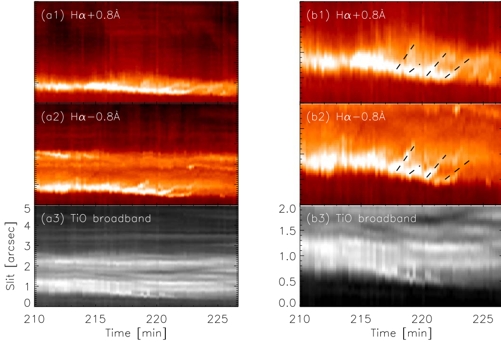
Figure 8. t - s plots derived from the TiO and H \alpha images along the curved slits in Figure 5(f) (left column) and enlarged t - s plots at y = 0'' – 2'' (right column). The black dashed lines in (b1)–(b2) mark the quasi-periodic bright blobs from the location of a vortex.
