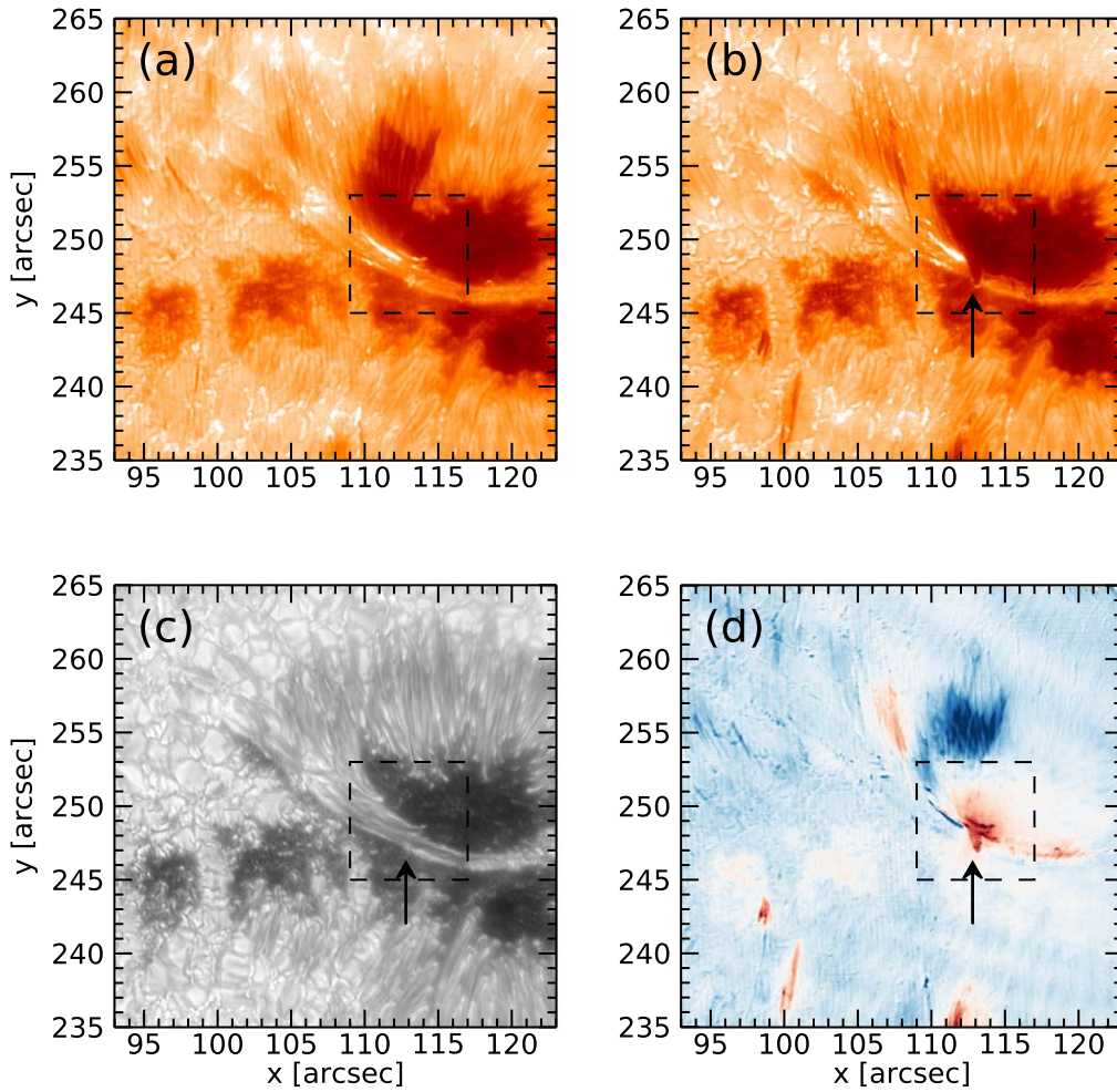
Figure 1. (a) Sunspot LB seen in the H\alpha wings at -0.8 \text{ \AA} , (b) +0.8 \text{ \AA} , (c) TiO, and (d) a H\alpha + 0.8 \text{ \AA} Doppler map at 16:24:13 UT. The x - and y -axes indicate distance from the disk center. The dashed box represents the FOV in Figure 5. This figure is accompanied by an animation that shows the temporal evolution of the region. The video begins in the TiO filter at 16:08:42. One can see transverse flows inside the light bridge. When the flow reaches the north and south edge of the LB, one of the filaments of the LB is protruding the umbra making a curled, vortex-like shape. At 17:00:01 the video zooms in on a vortex moving ahead with the photospheric flow on the sunspot light bridge. The video continues in the TiO filter until 18:02:43 when the filter changes to the H\alpha wings at +0.8 \text{ \AA} until 18:17:43. 26 s into the video, when it begins to cycle between a single frame from the H\alpha wings at +0.8 \text{ \AA} , H\alpha wings at -0.8 \text{ \AA} , composite H\alpha wings at \pm 0.8 \text{ \AA} , TiO, and finally back to H\alpha wings at +0.8 \text{ \AA} . The sequence resumes 44 s in H\alpha wings at +0.8 \text{ \AA} and runs until 18:38:59. At the 18:41:33 the H\alpha wings at the \pm 0.8 \text{ \AA} filter are shown as the animation pans outward. The video ends at 19:59:01. Its total duration is 1 minute.
